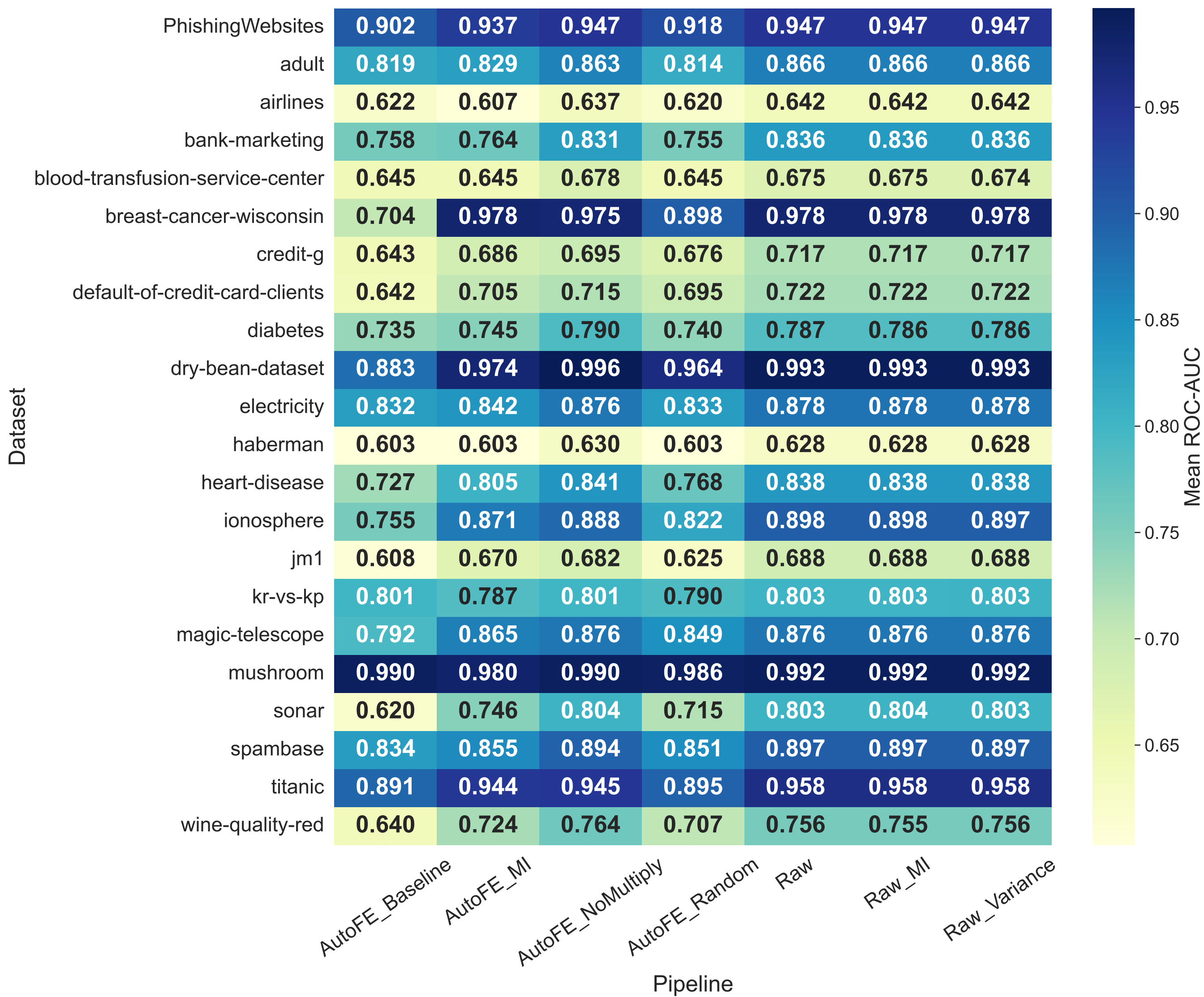
Figure 9: Dataset vs Pipeline Performance Heatmap
