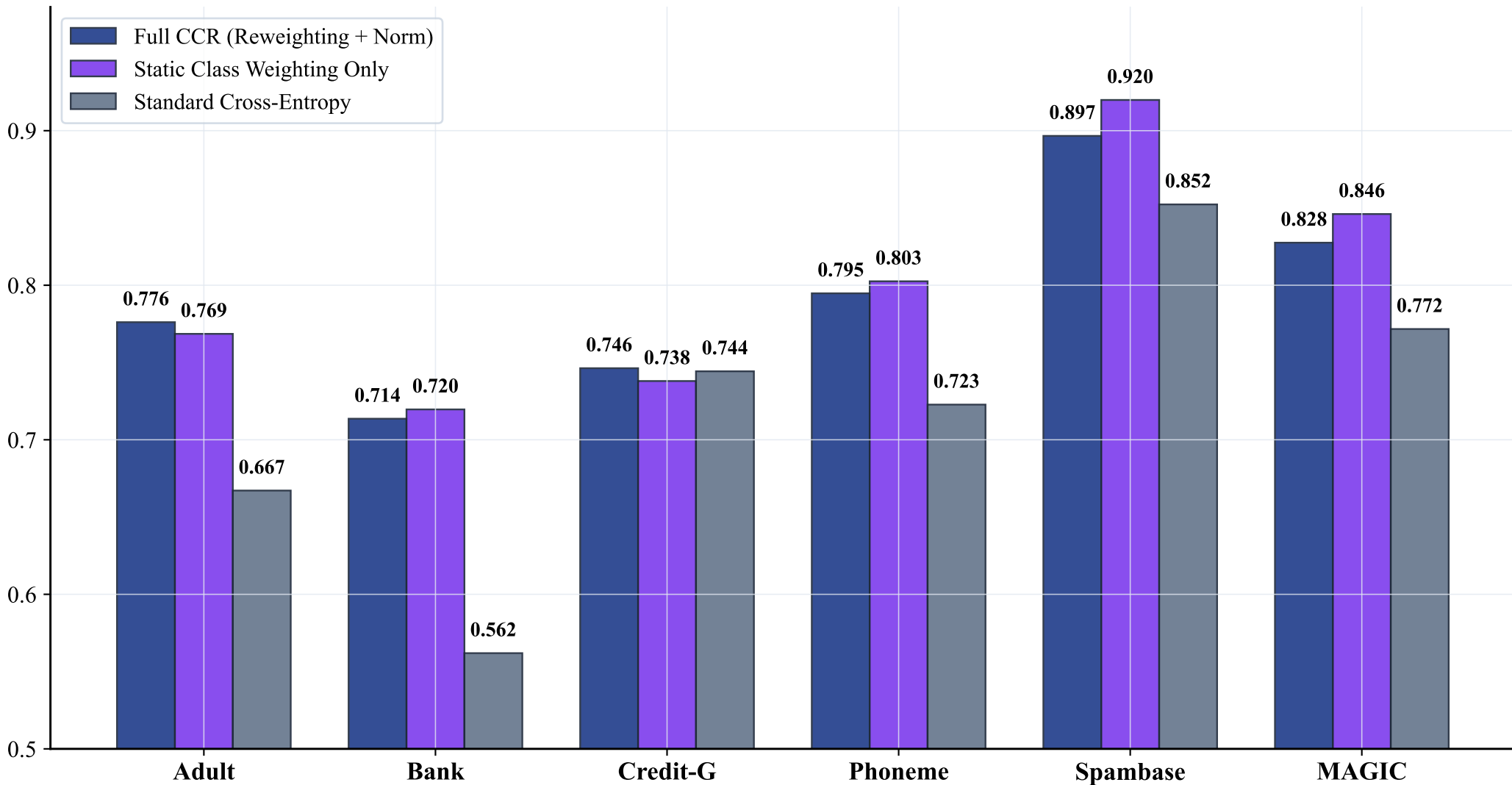
Macro-F1 Score at 40% Noise
