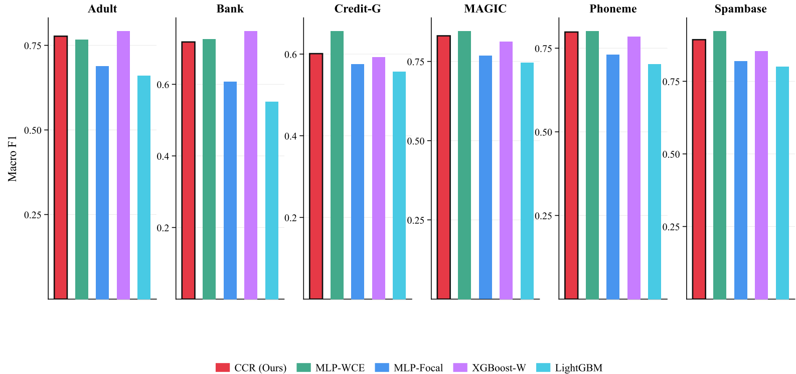
Macro F1 at Extreme Noise (Asymmetric 40%)
