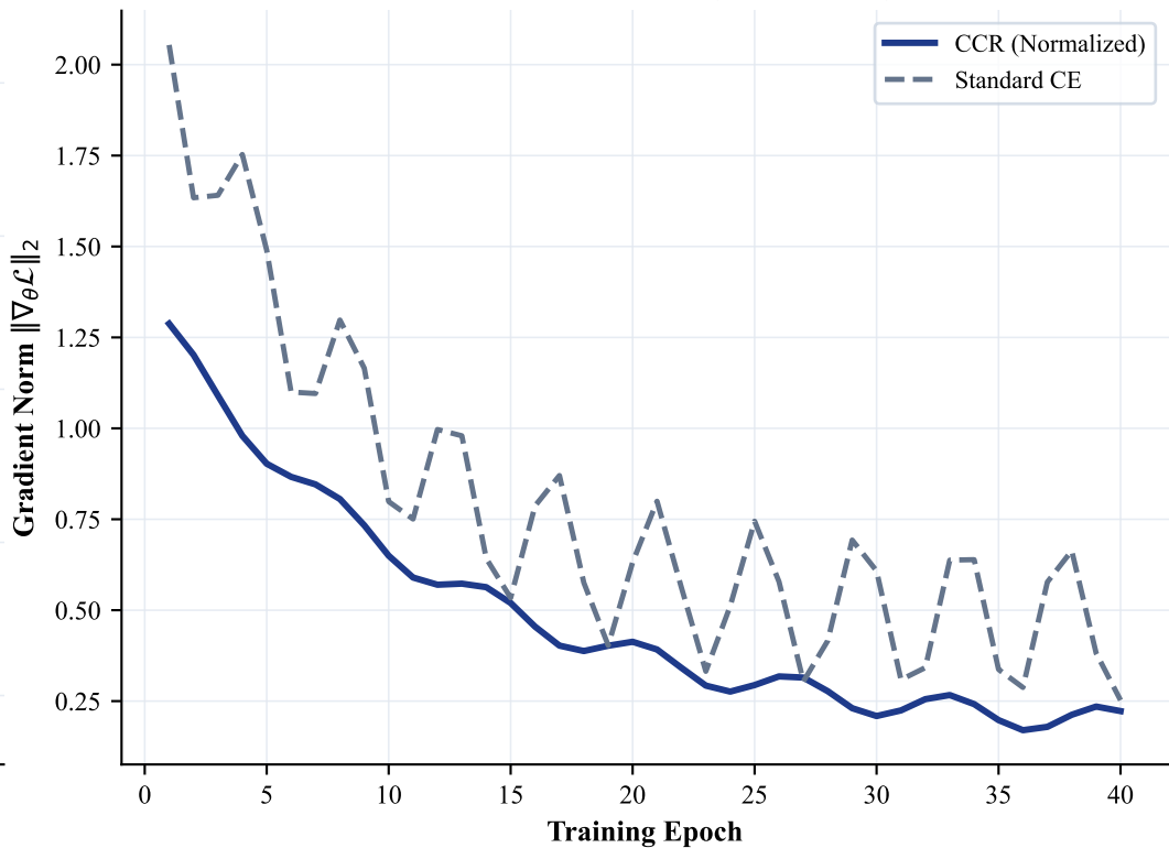
Gradient Norm Stability & Volatility
