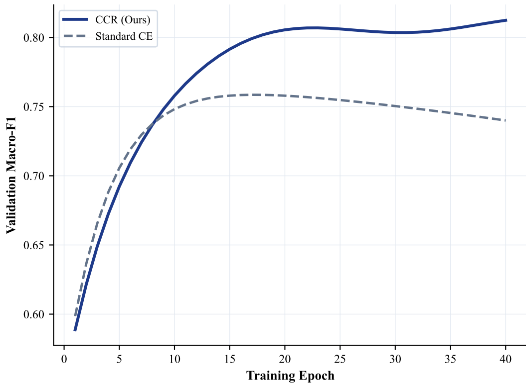
Validation Robustness Dynamics (40% Noise)
