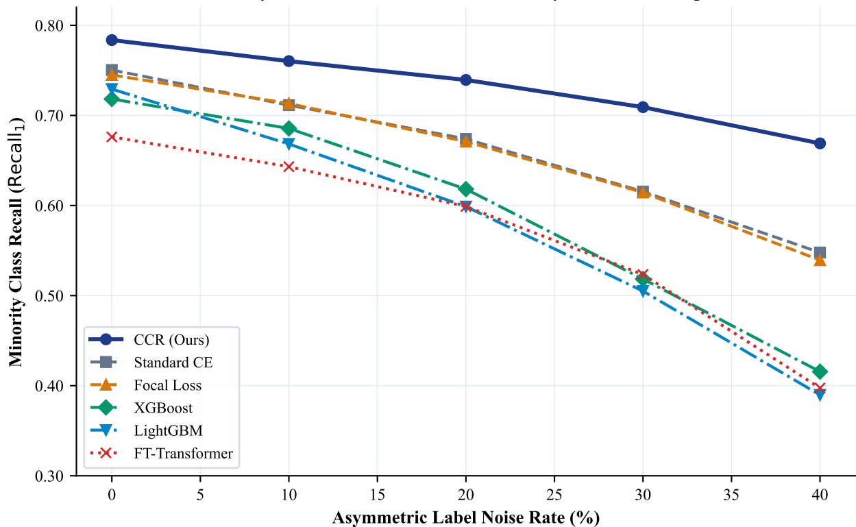
Minority-Class Recall Retention under Asymmetric Corruption
