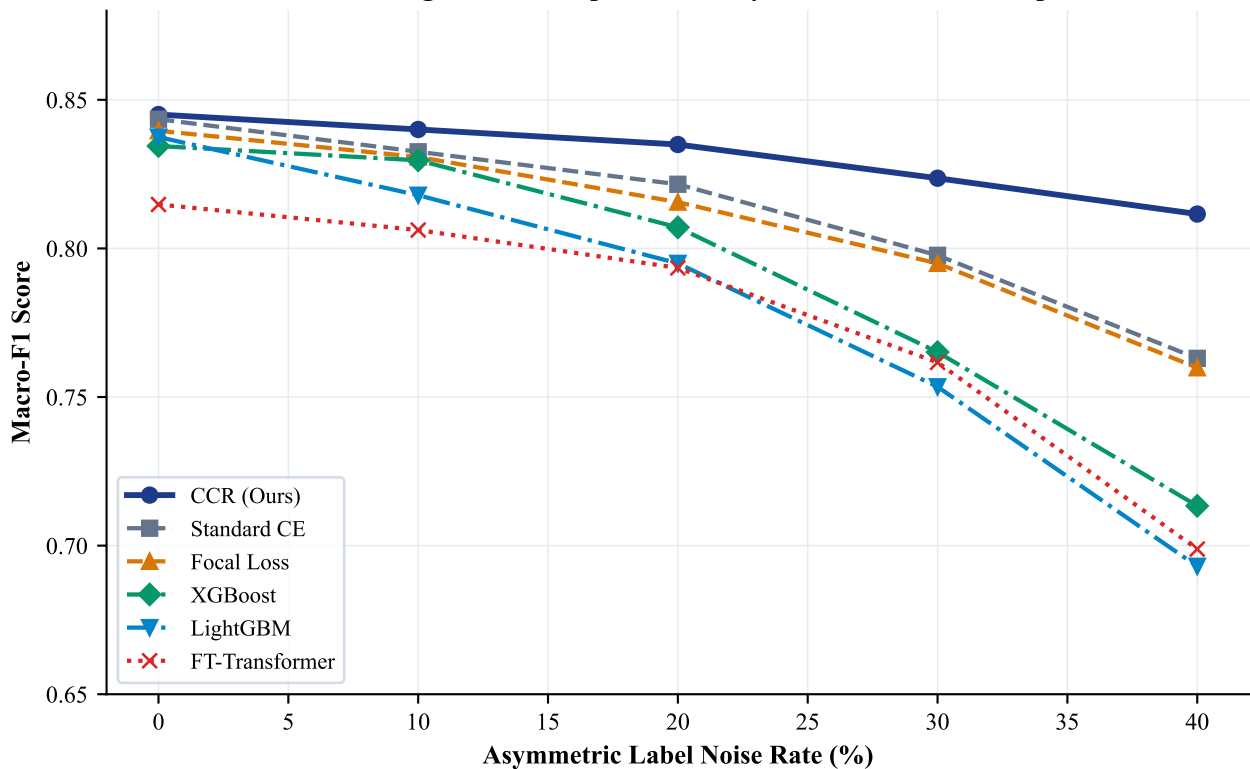
Macro-F1 Degradation Slopes under Asymmetric Label Corruption
