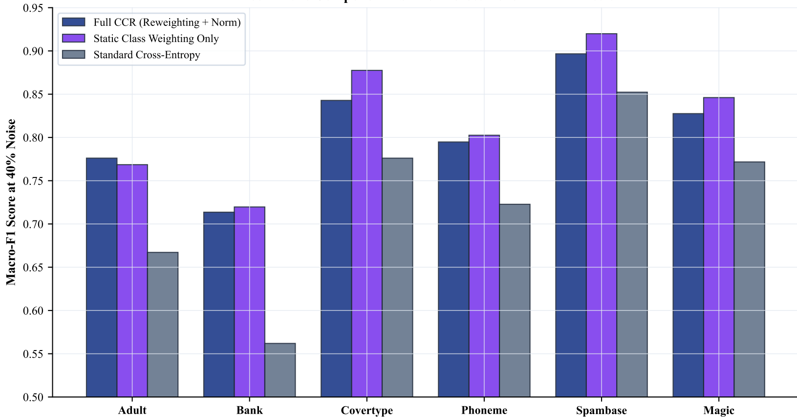
Mechanistic Component Ablation across Benchmark Datasets
