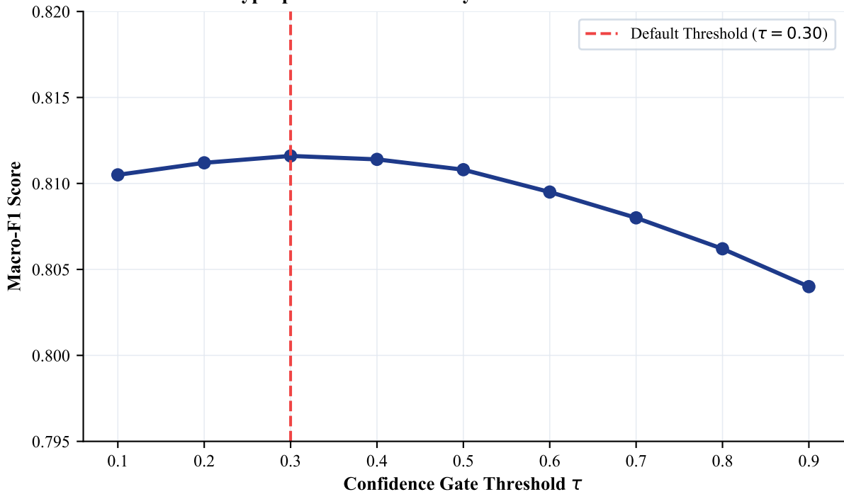
Hyperparameter Sensitivity: Confidence Threshold \tau
