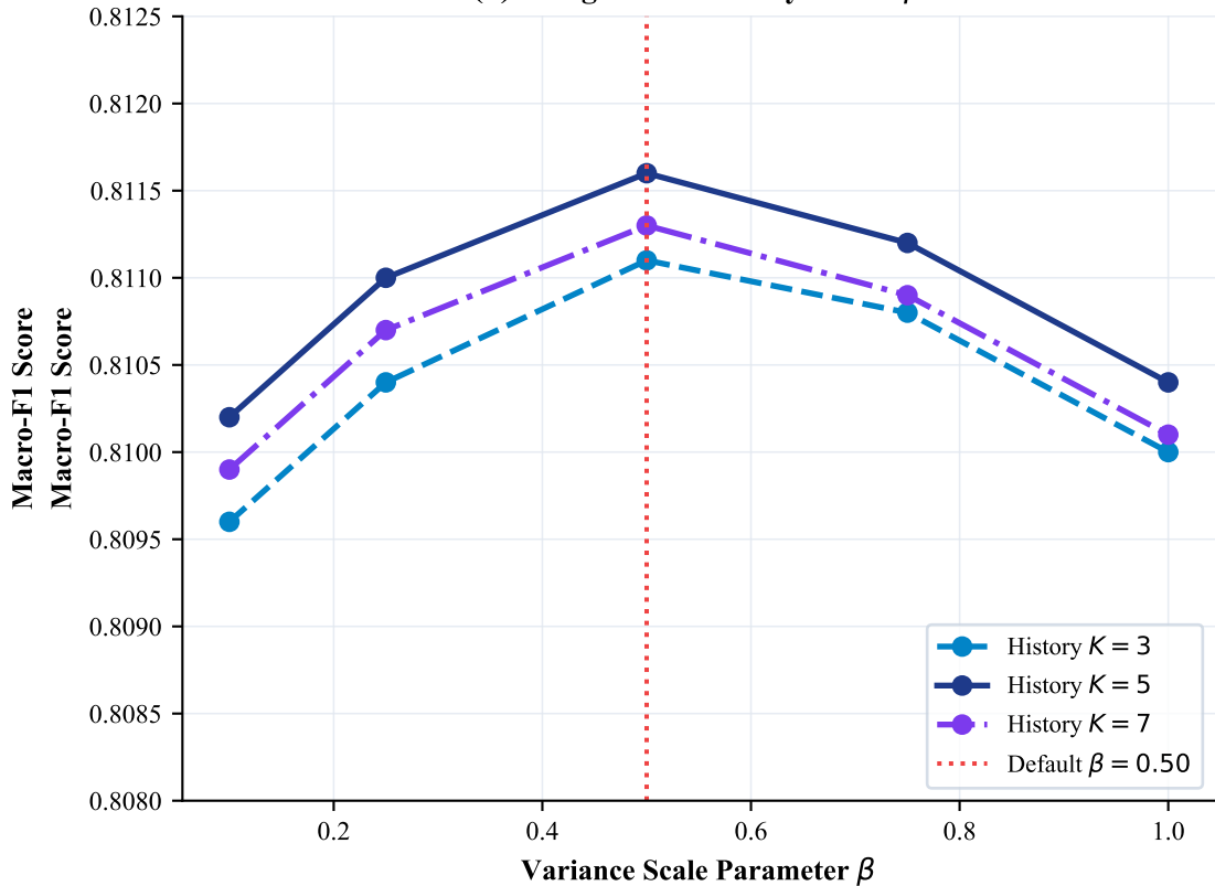
(b) Marginal Sensitivity across \beta
