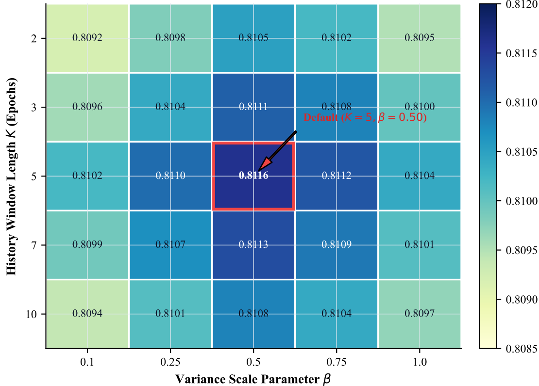
(a) 2D Grid Sweep: K vs. \beta
