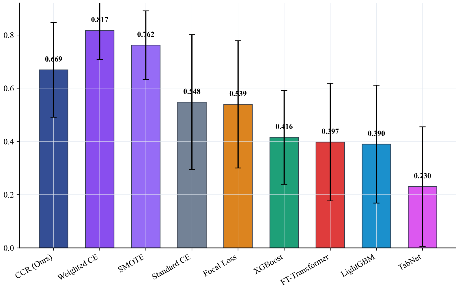
Minority Class Recall (Recall 1 )
