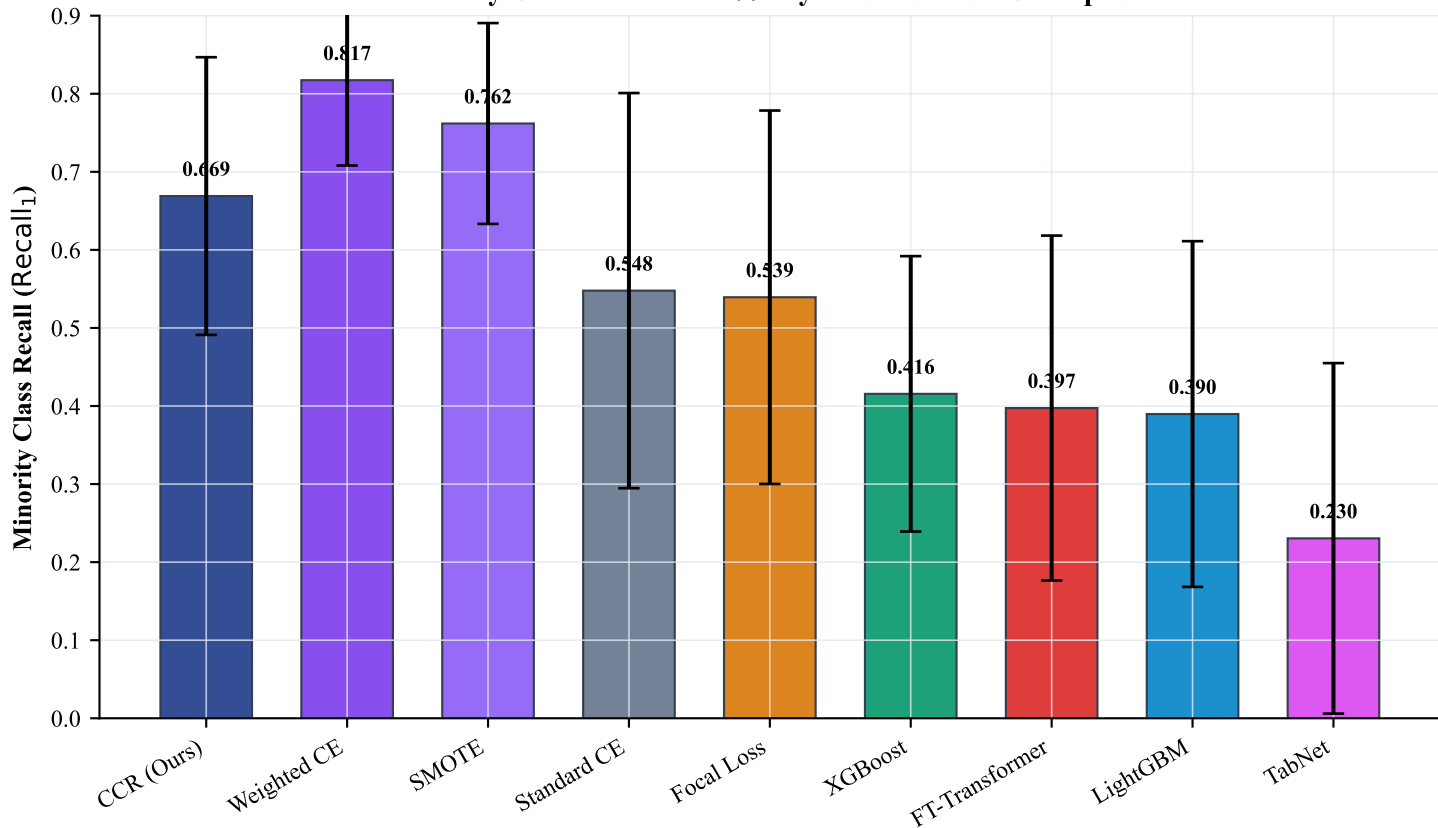
Minority Class Recall at 40% Asymmetric Label Corruption
