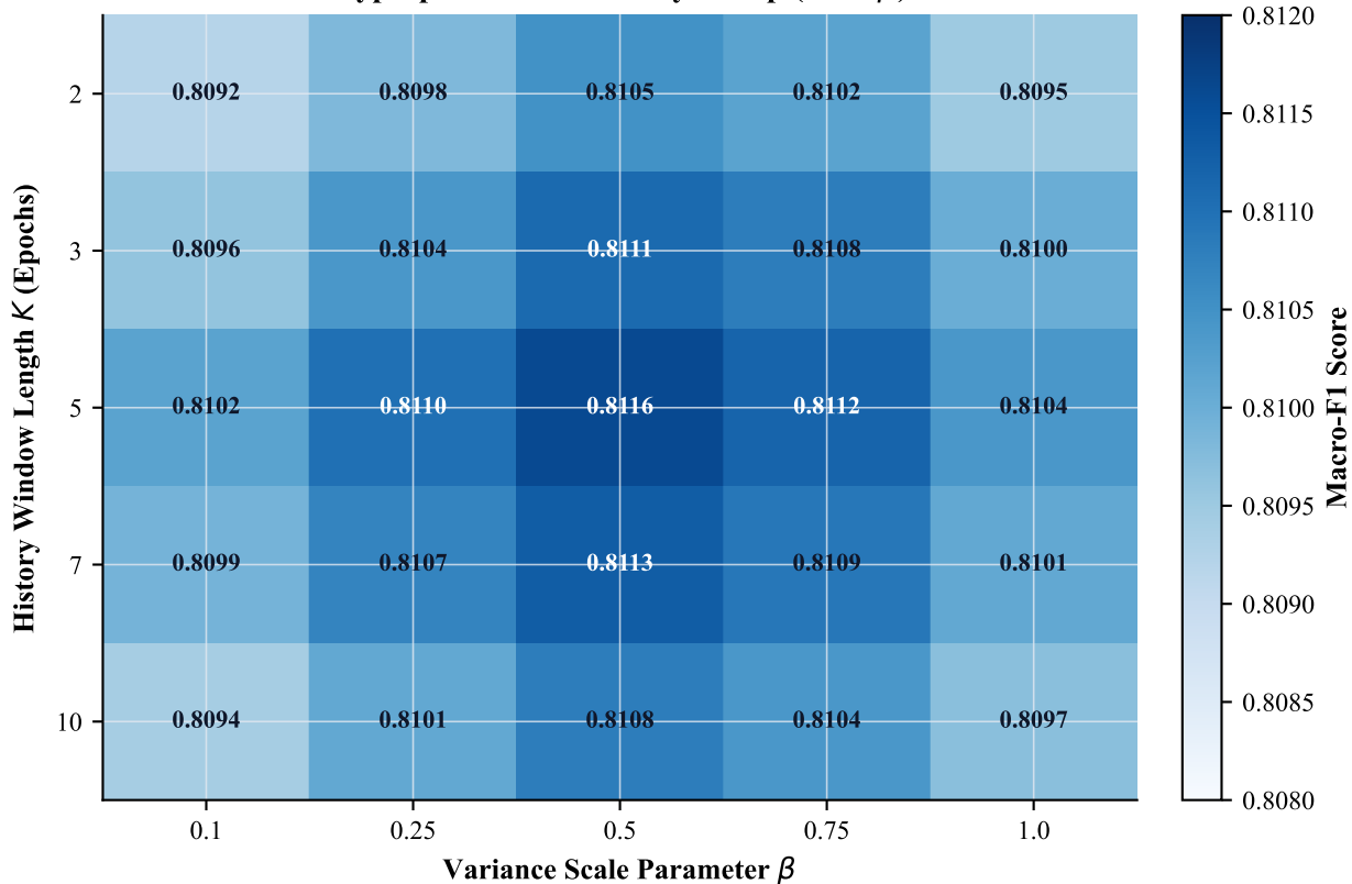
Hyperparameter Stability Sweep ( K vs. \beta )
