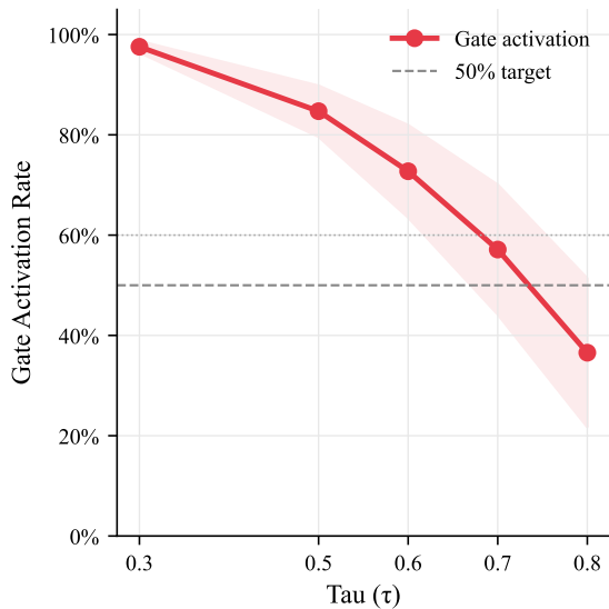
Gate Activation vs \tau
