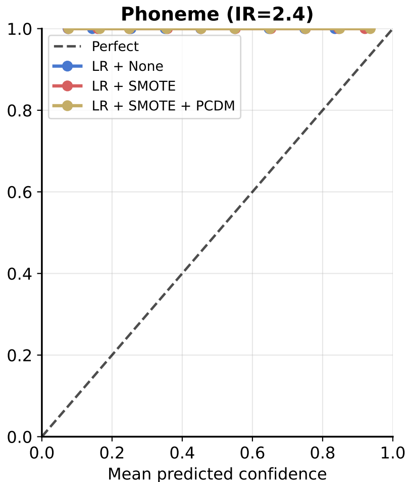
Appendix Figure A — Minority-Class Reliability Diagrams (5 seeds) Shaded band = \pm 1 std
