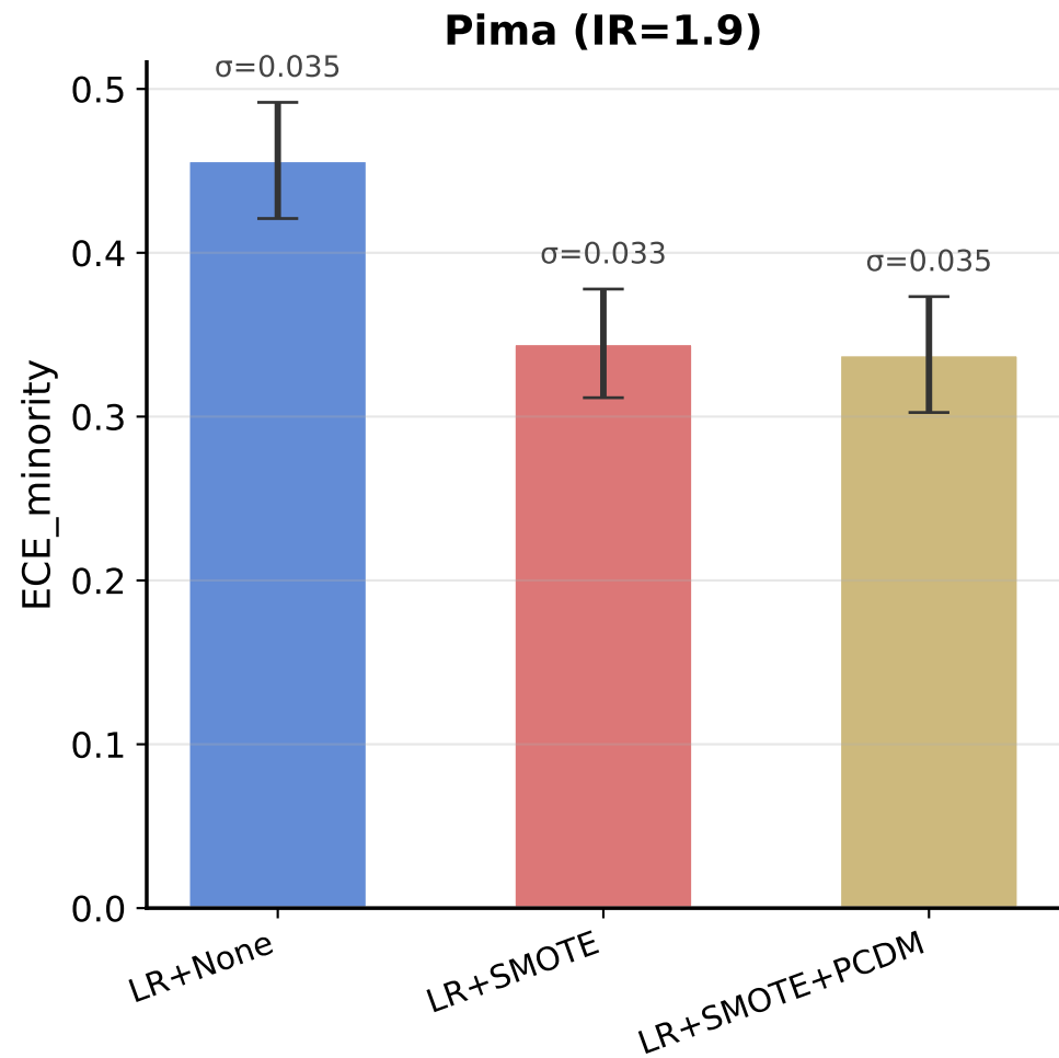
Appendix Figure B — ECE_minority Variance Across 5 Seeds Error bars = \pm 1 std
