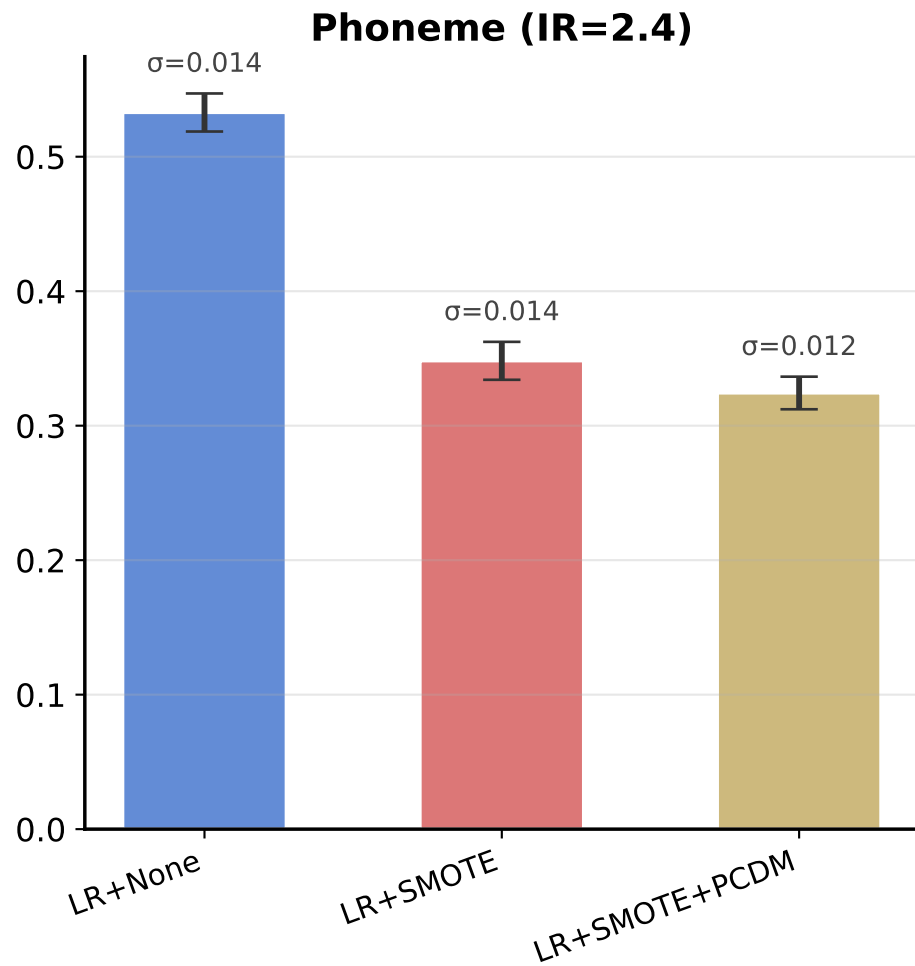
Appendix Figure B — ECE_minority Variance Across 5 Seeds Error bars = \pm 1 std
