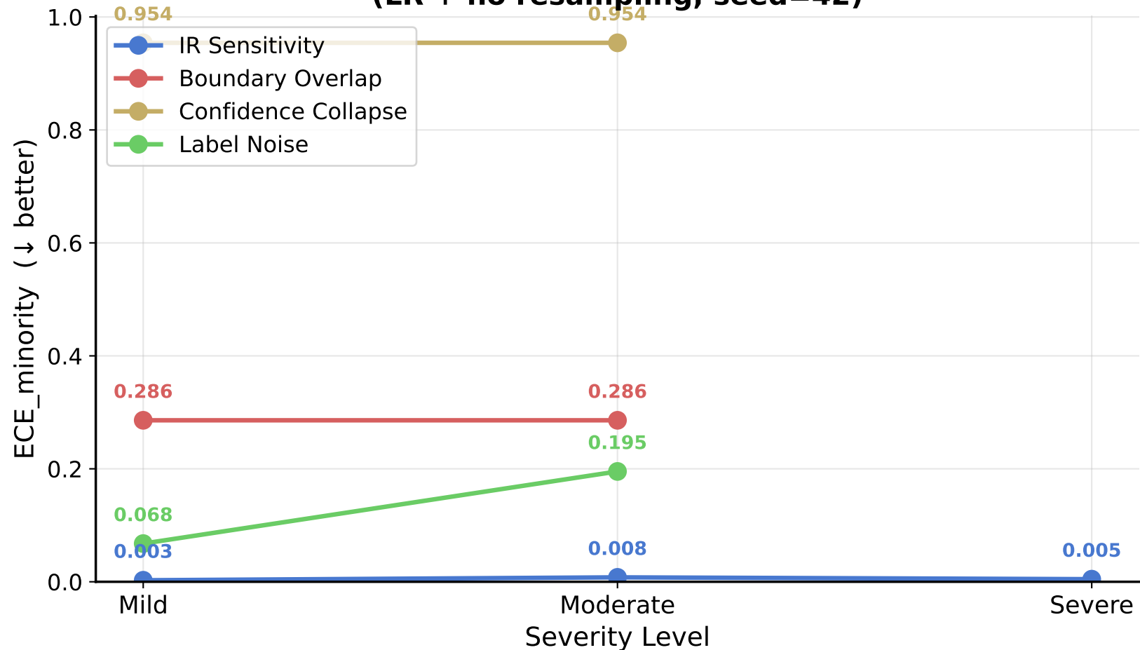
Figure 4 — Calibration Degradation Across Severity Levels (LR + no resampling, seed=42)
