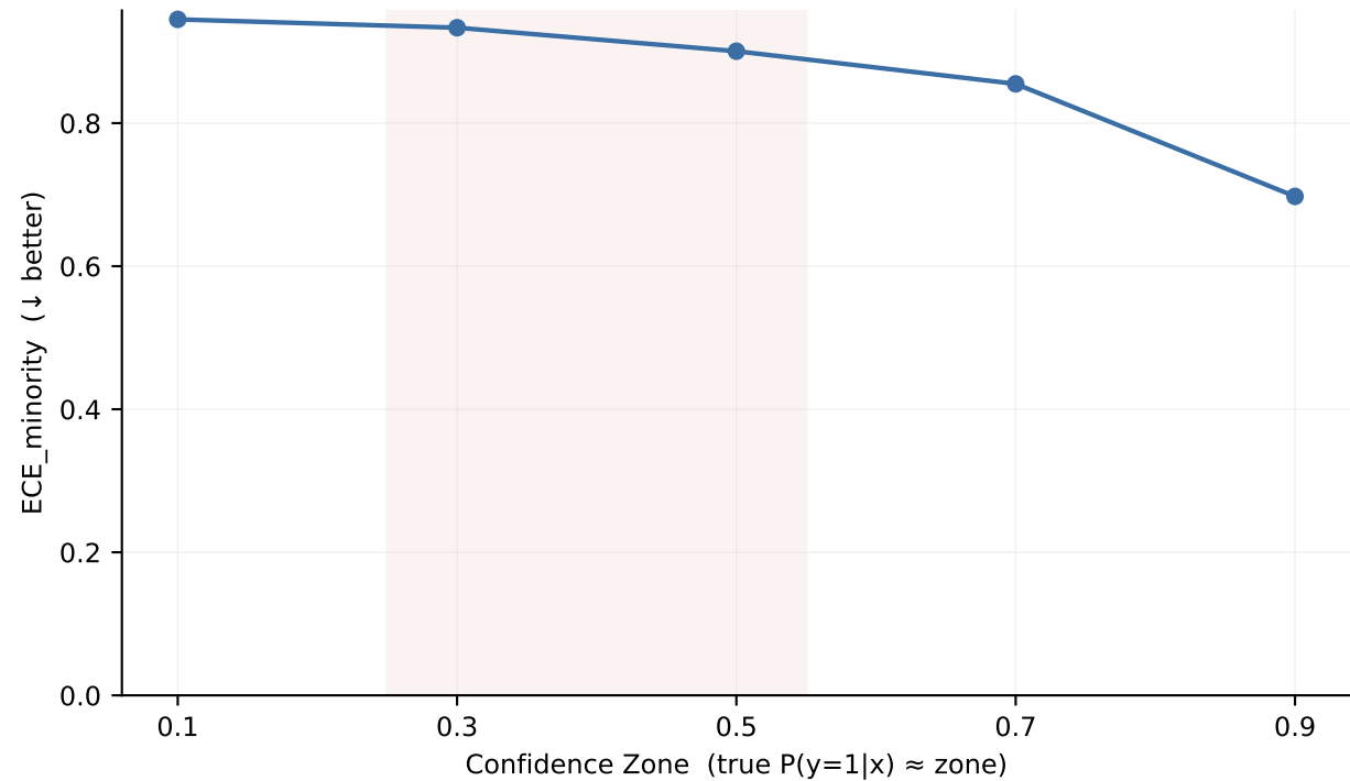
Figure 5 — Calibration Error Across Confidence Zones (shaded region = instability zone, LR + no resampling)
