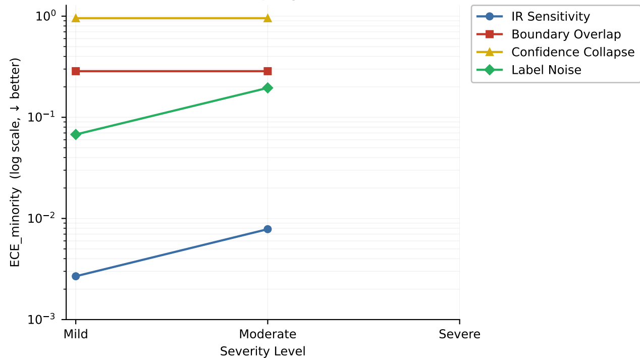
Figure 4 — Calibration Degradation Across Severity Levels (LR + no resampling, seed=42)
