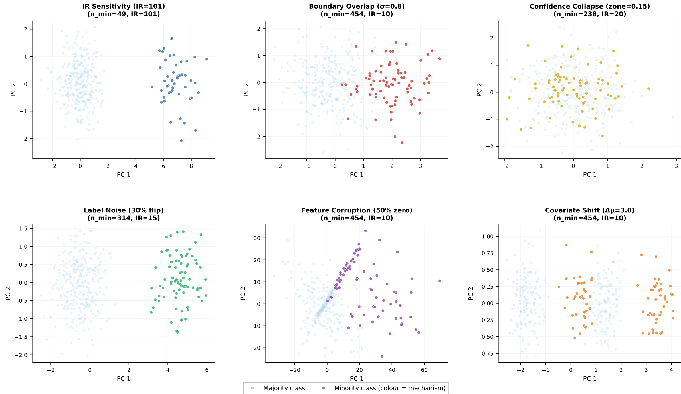
Figure 6 — Calibration Stress Test Suite (PCA projection, severe severity, seed=42)
