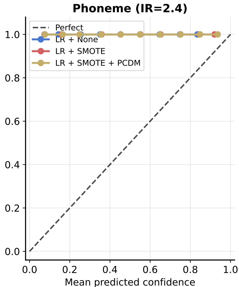
Appendix Figure A — Minority-Class Reliability Diagrams (5 seeds) Shaded band = \pm 1 std
