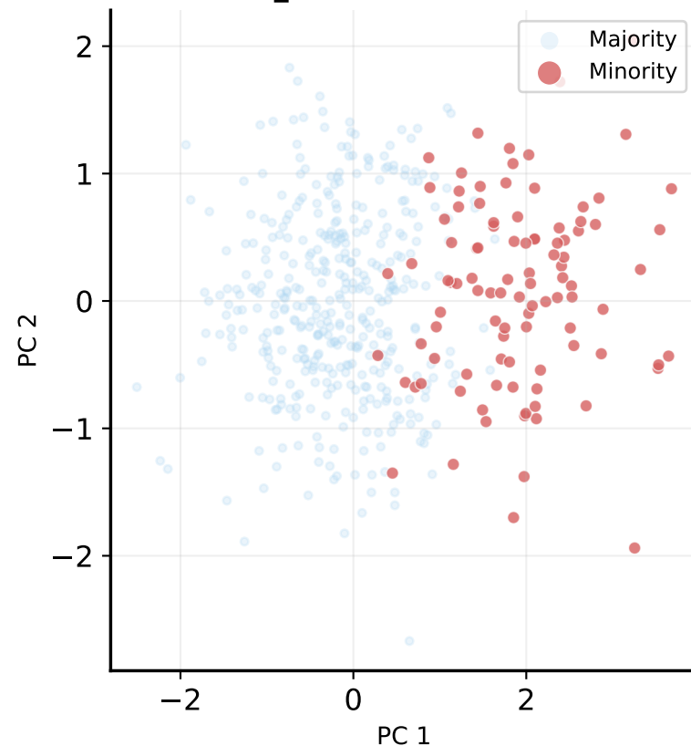
Boundary Overlap ( \sigma=0.8 ) n_min=454, IR=10
