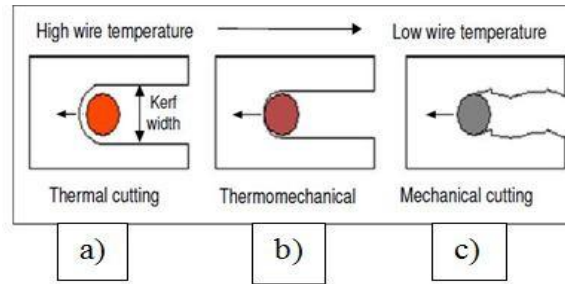
Fig. 1. Cutting mechanisms
