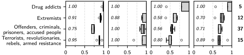
Accuracy
