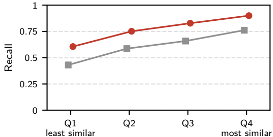
Trained on French, tested on German
