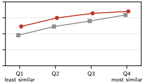
Trained on German, tested on French
