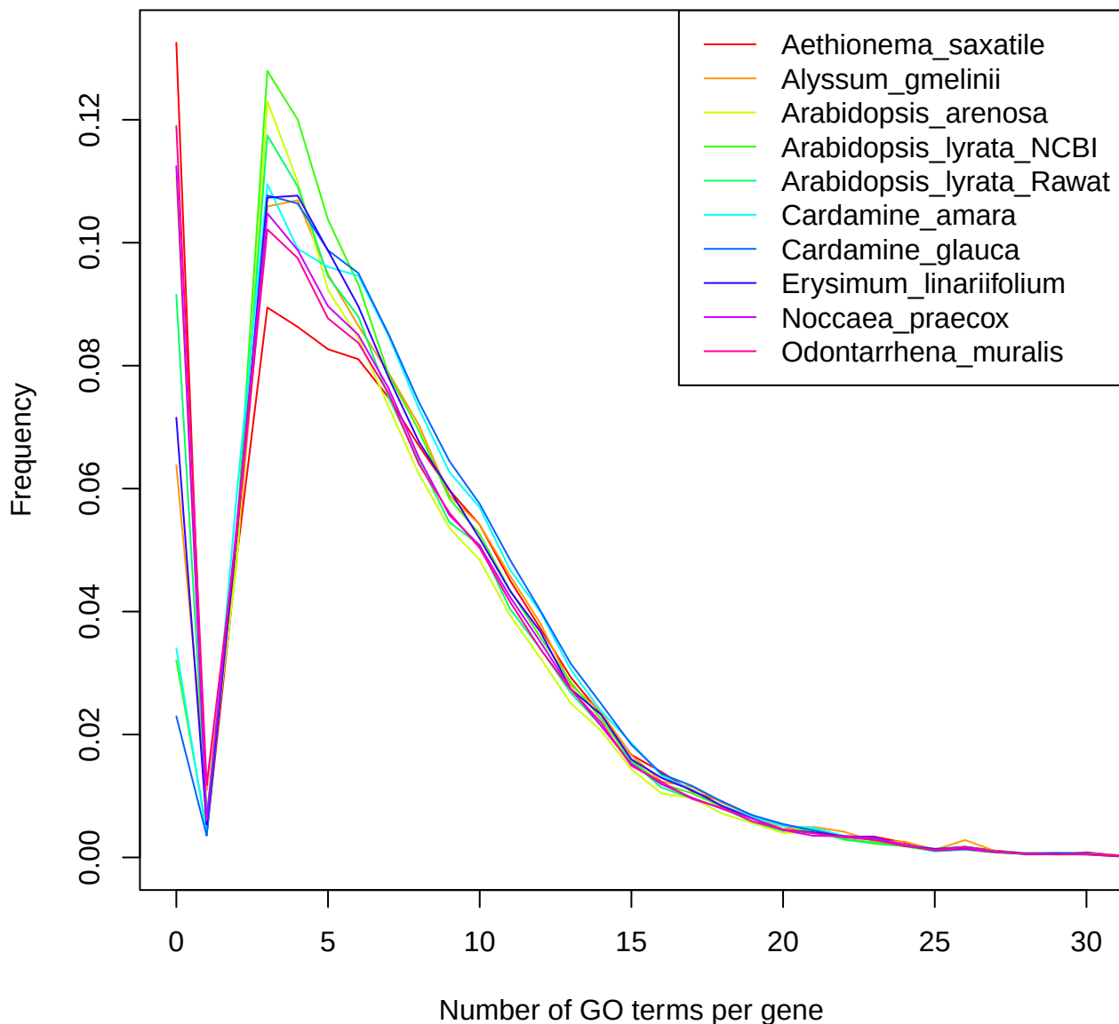
Number of GO terms per gene
