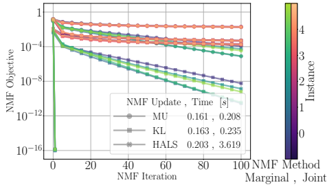
(c) Bond dimension \chi = 8
