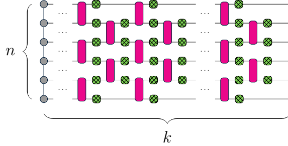
Figure 6.8: Brickwork quantum circuits. k layers of n component brickwork layouts of unitaries (pink) and local noise (green).
