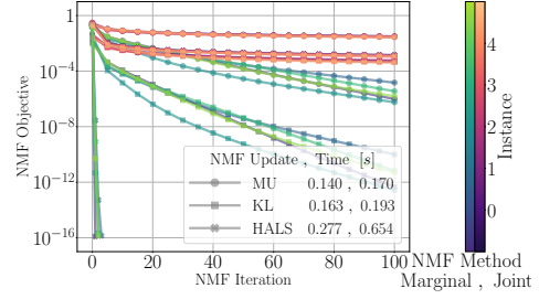
(b) Bond dimension \chi = 4
