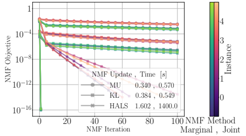
(f) Bond dimension \chi = 64
