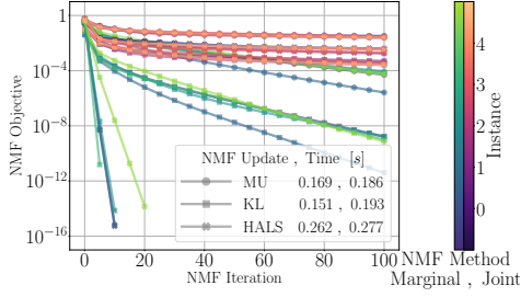
(a) Bond dimension \chi = 2
