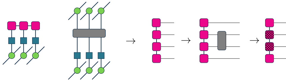
Figure 6.4: POVM-MPS architecture. States \rho (left) and channels \Lambda (centre) can be expanded in terms of local operators \Pi \in \mathcal{P} (green circles), with inverse overlap matrices \chi_{\mathcal{P}}^{-1} (blue squares), and probabilities p (pink squares). Probabilities can be represented as stochastic matrix product states (right), which can be updated to p \rightarrow p' (pink-hatched squares) with quasi-stochastic matrices L (gray rectangles) associated with \Lambda .
