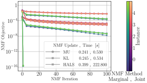
(e) Bond dimension \chi = 32
