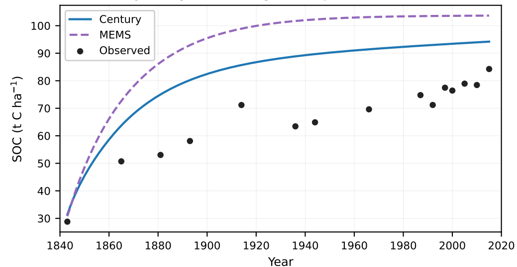
d SOC trajectory, FYM (long-term qualitative)
