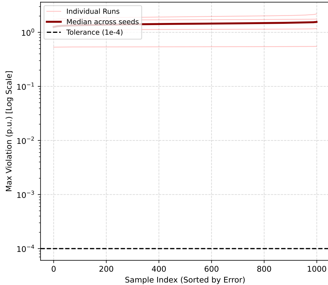
KKT (5 seeds)
