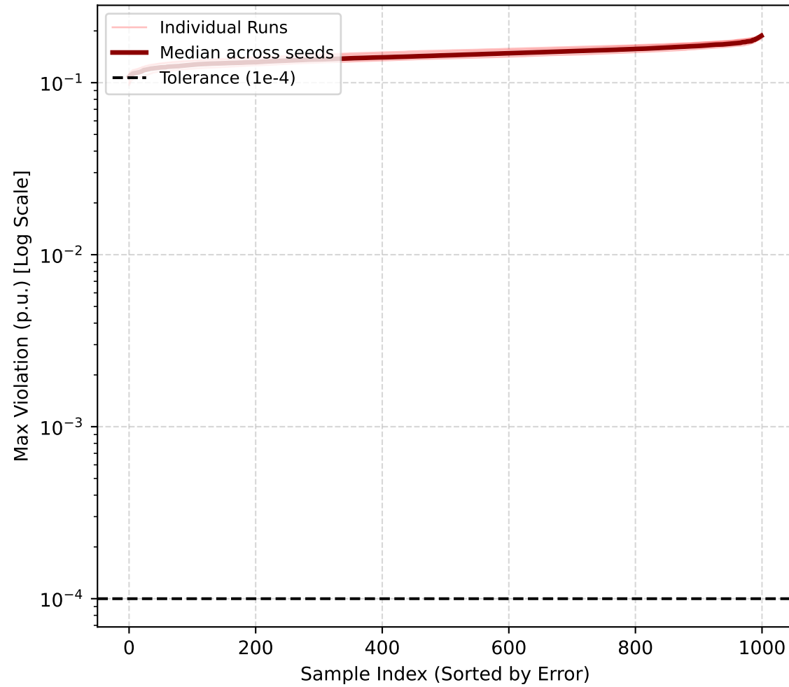
KKT (5 seeds)
