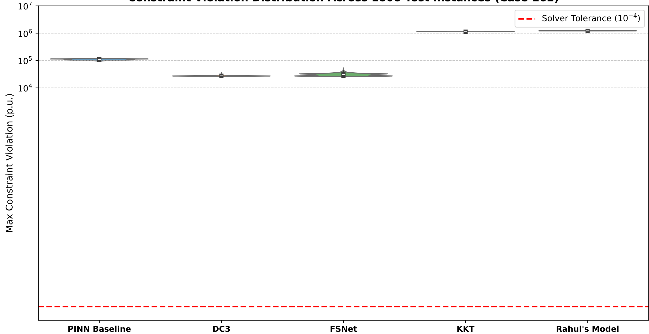
Constraint Violation Distribution Across 1000 Test Instances (Case 162)
