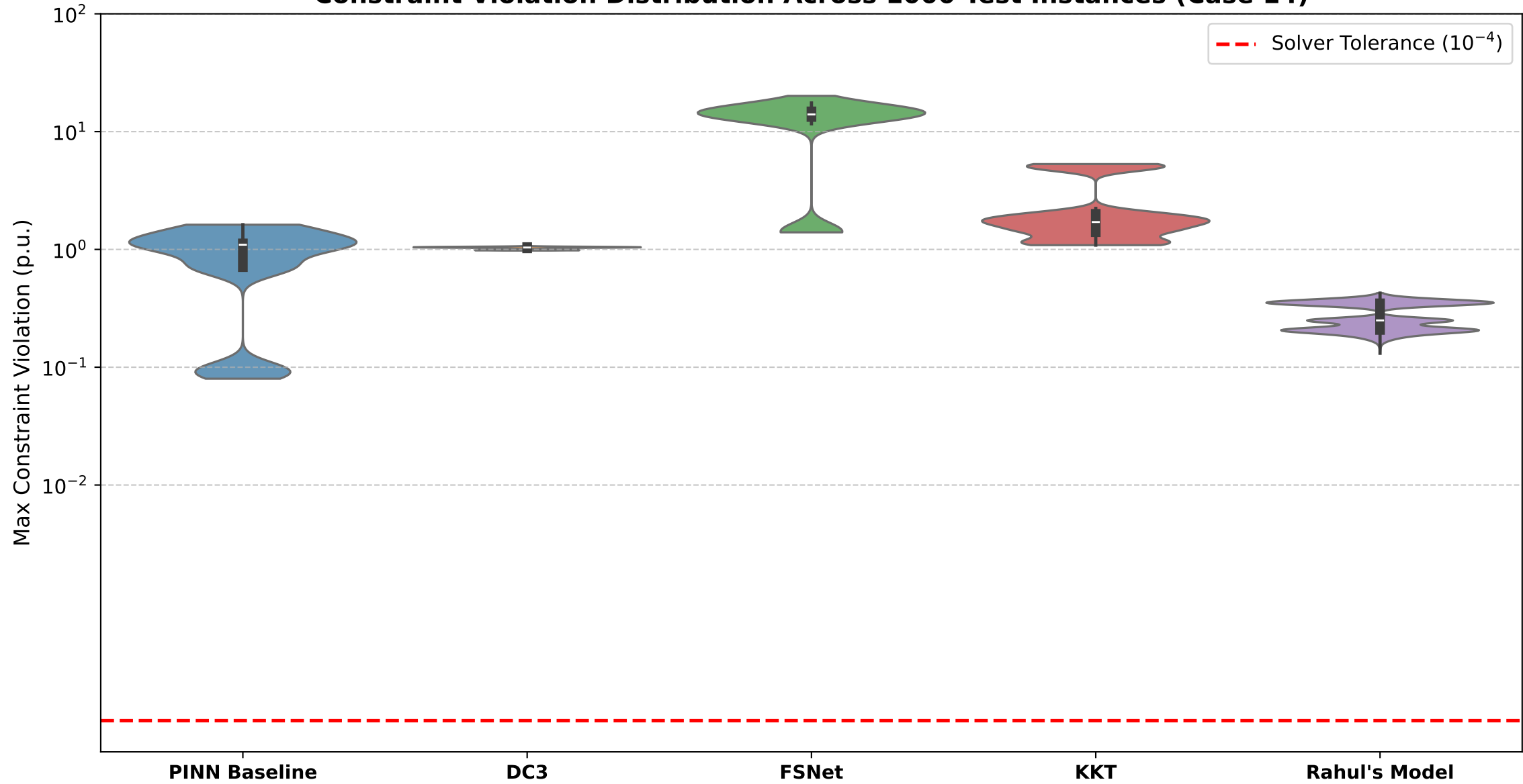
Constraint Violation Distribution Across 1000 Test Instances (Case 14)
