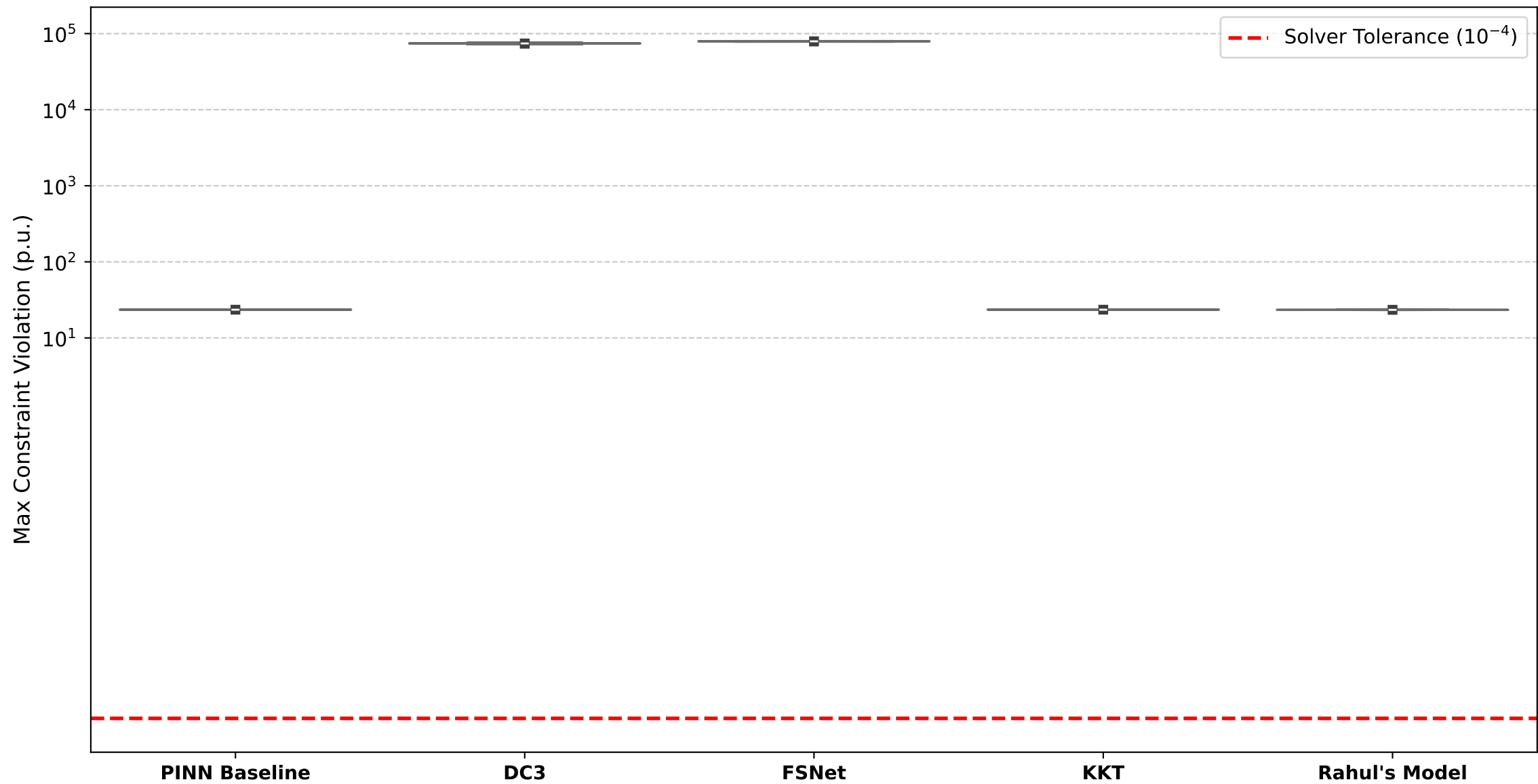
Constraint Violation Distribution Across 1000 Test Instances (Case 300)
