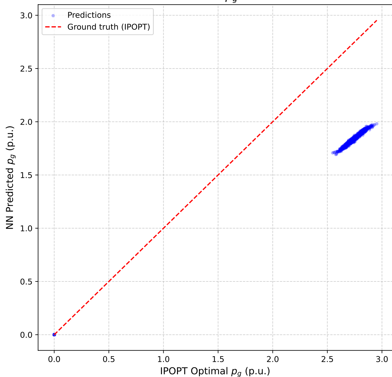
FSNet Model: p_g vs IPOPT
