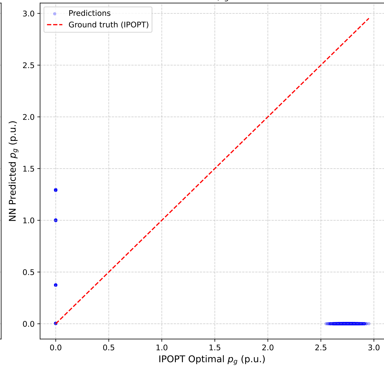
Rahul Model: p_g vs IPOPT
