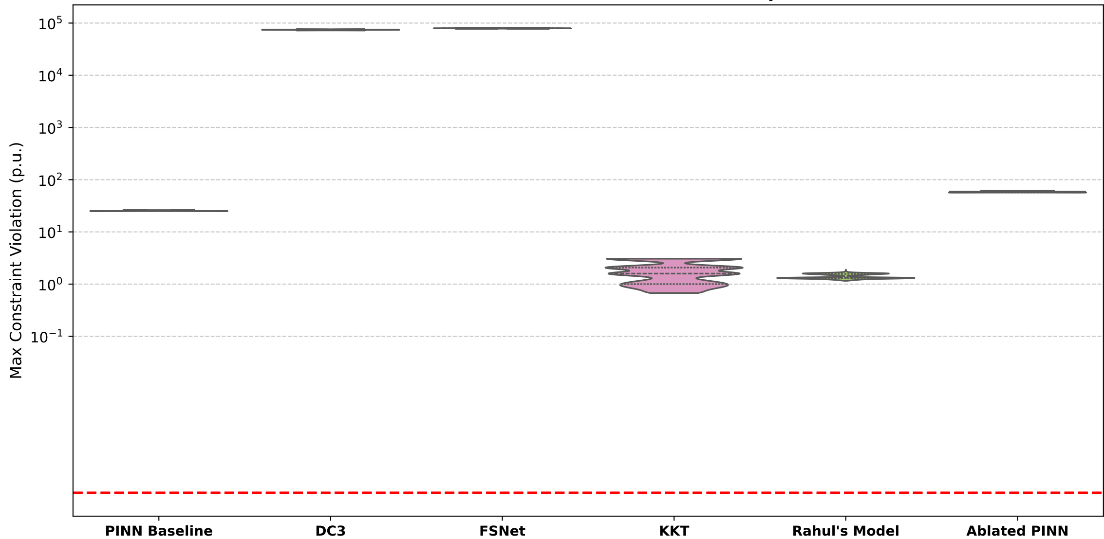
Maximum Constraint Violations: 300-Bus Case Pooled across 5 runs (1,000 test instances per run)
