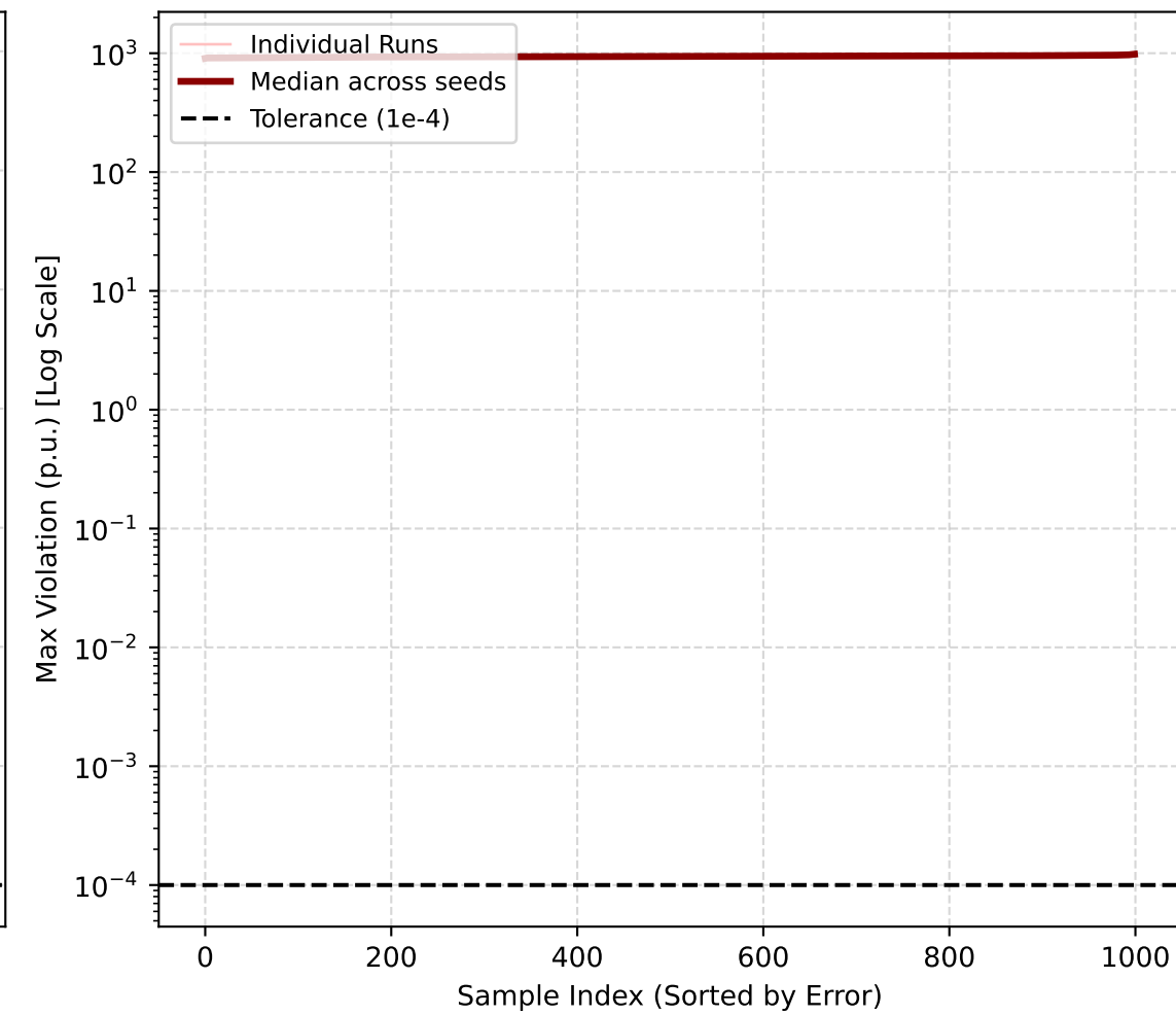
FSNet (5 seeds)
