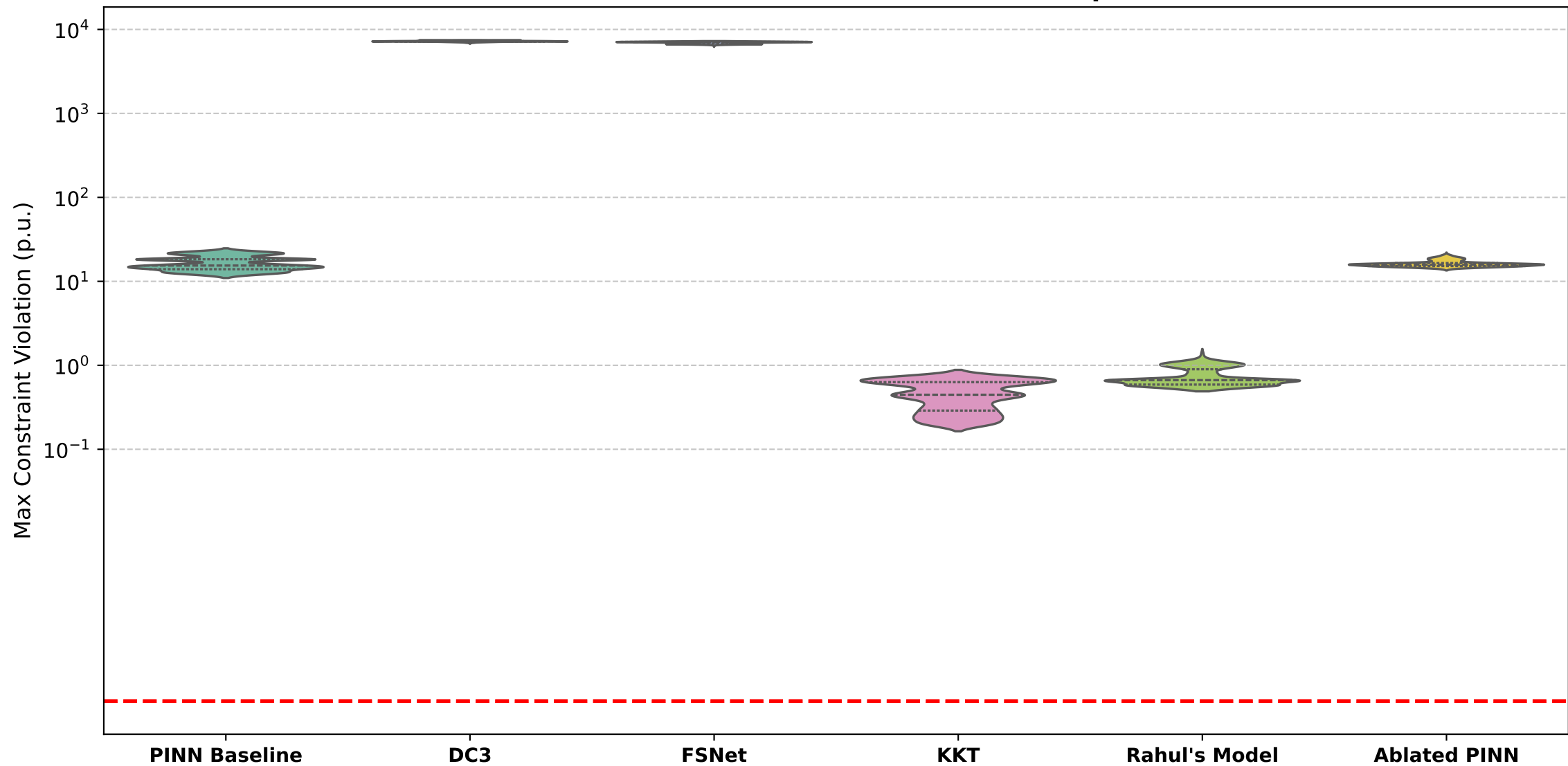
Maximum Constraint Violations: 162-Bus Case Pooled across 5 runs (1,000 test instances per run)
