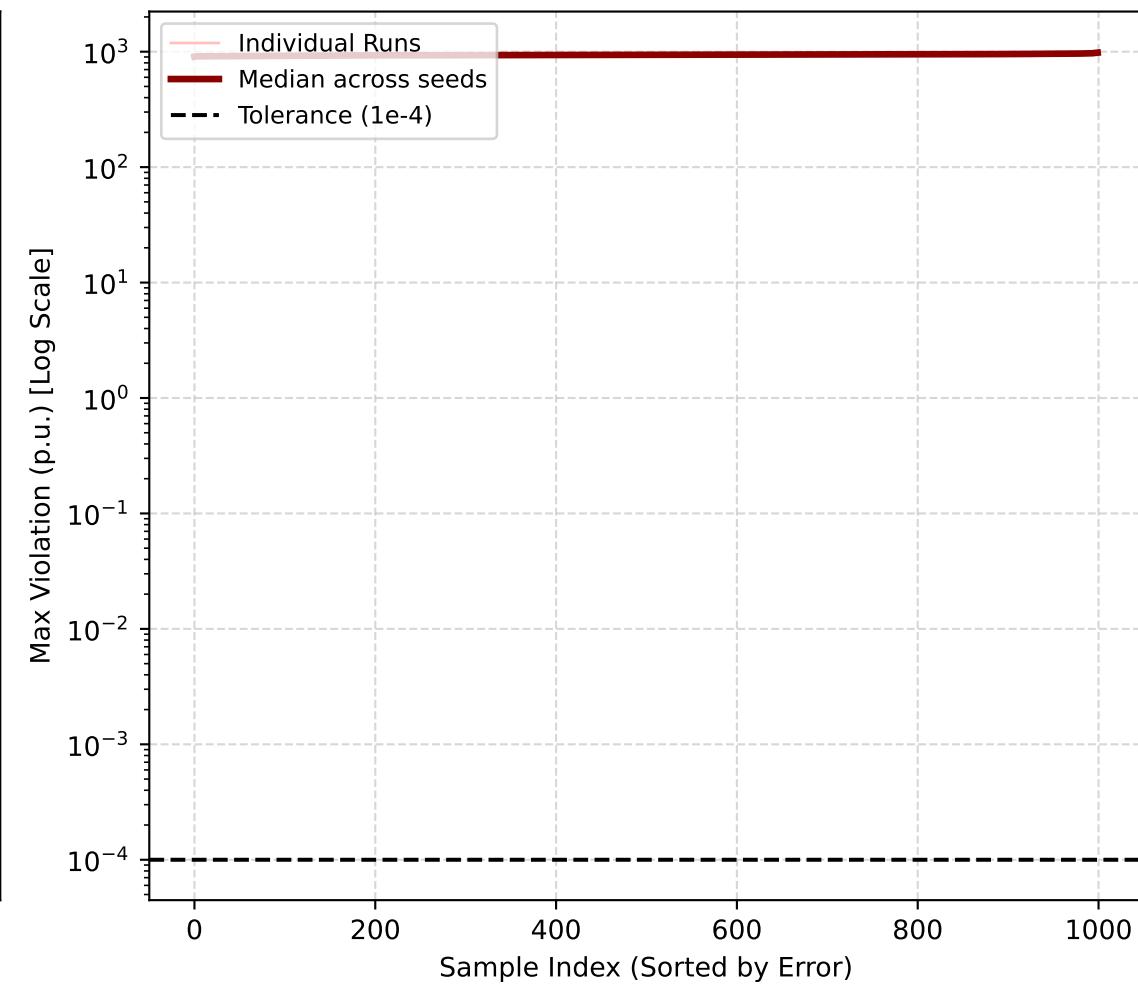
Ablated PINN (5 seeds)
