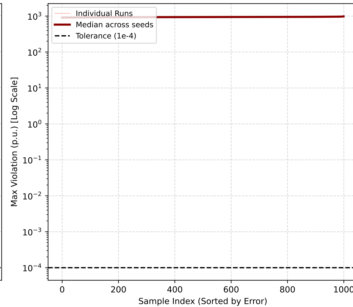
Ablated PINN (5 seeds)
