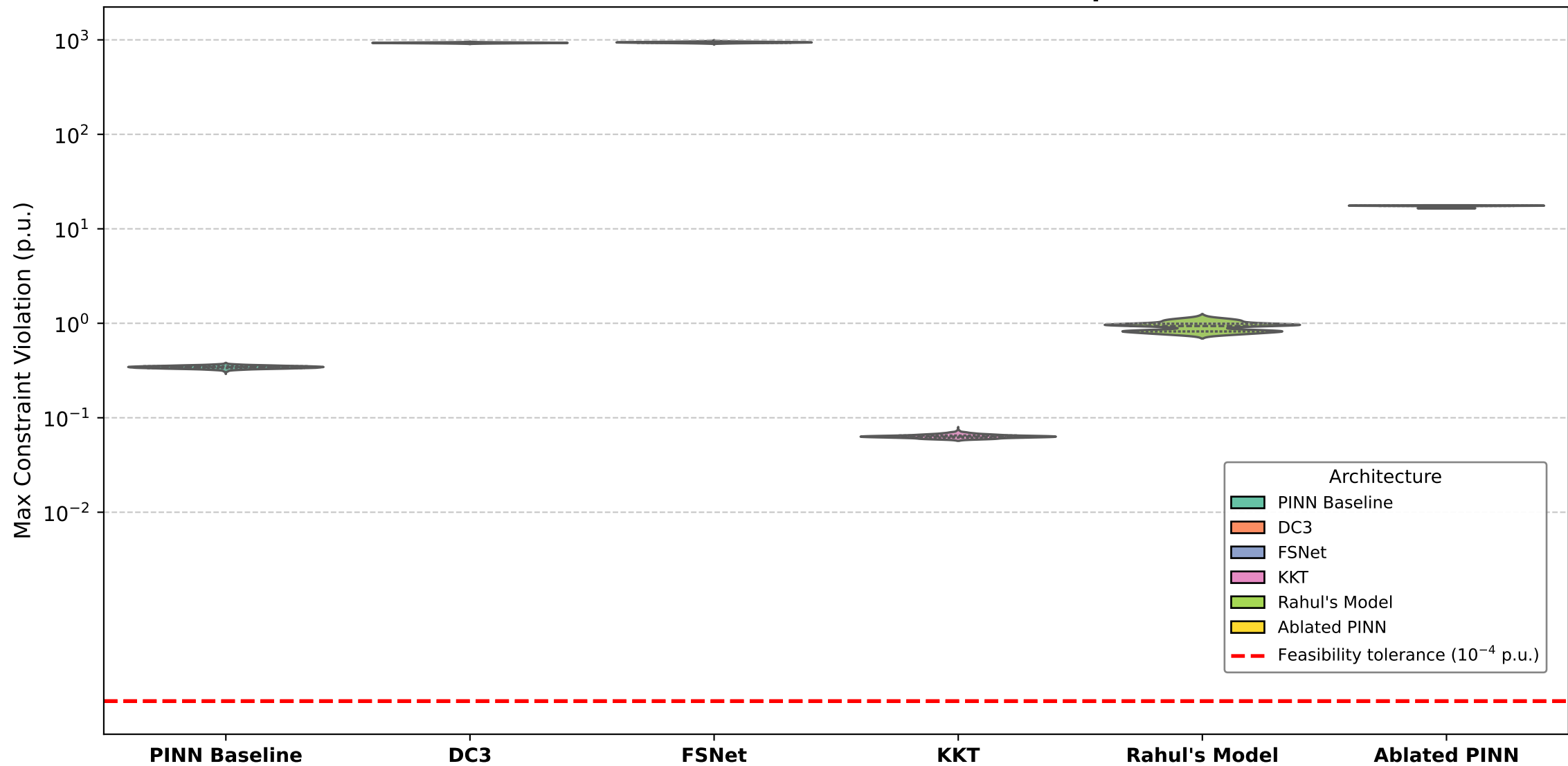
Maximum Constraint Violations: 57-Bus Case Pooled across 5 runs (1,000 test instances per run)
