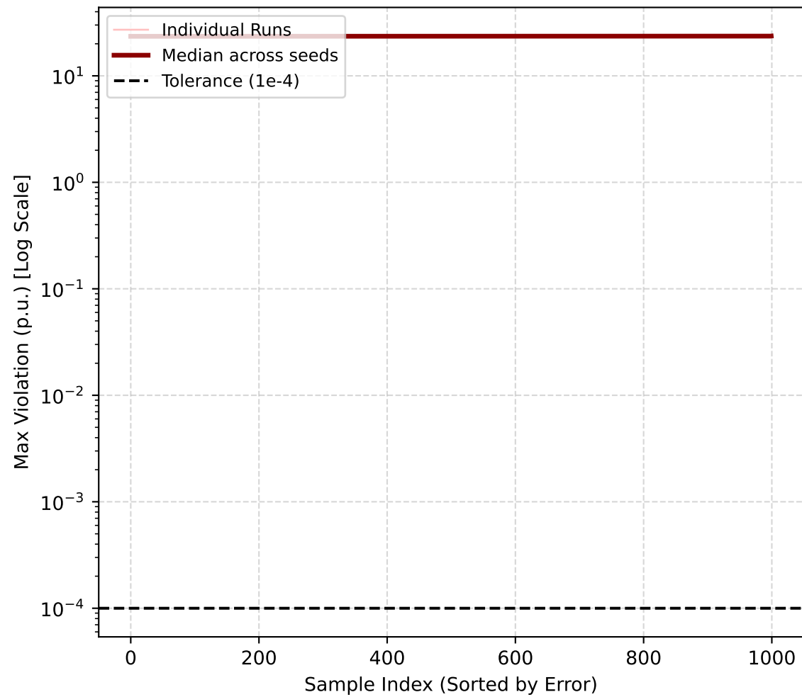
KKT (5 seeds)
