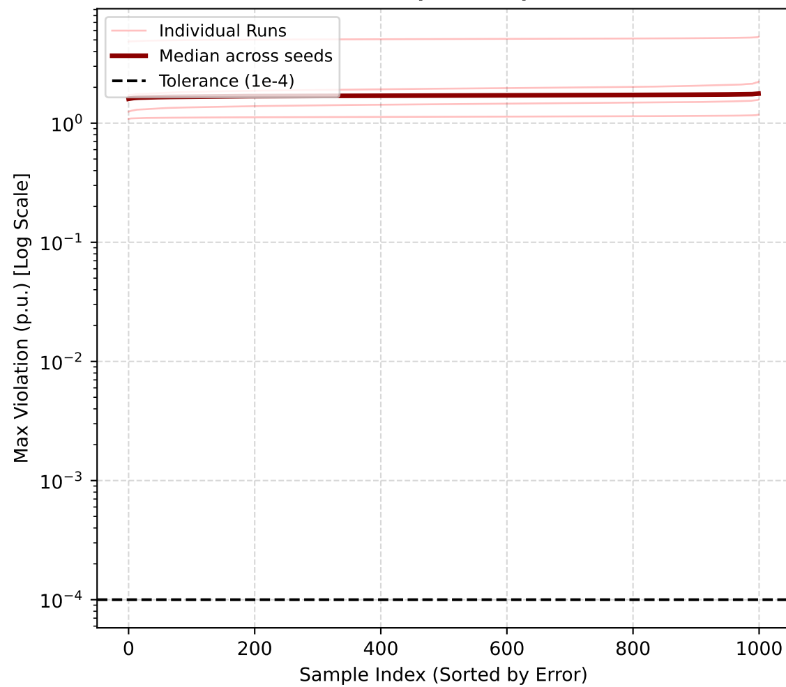
KKT (5 seeds)
