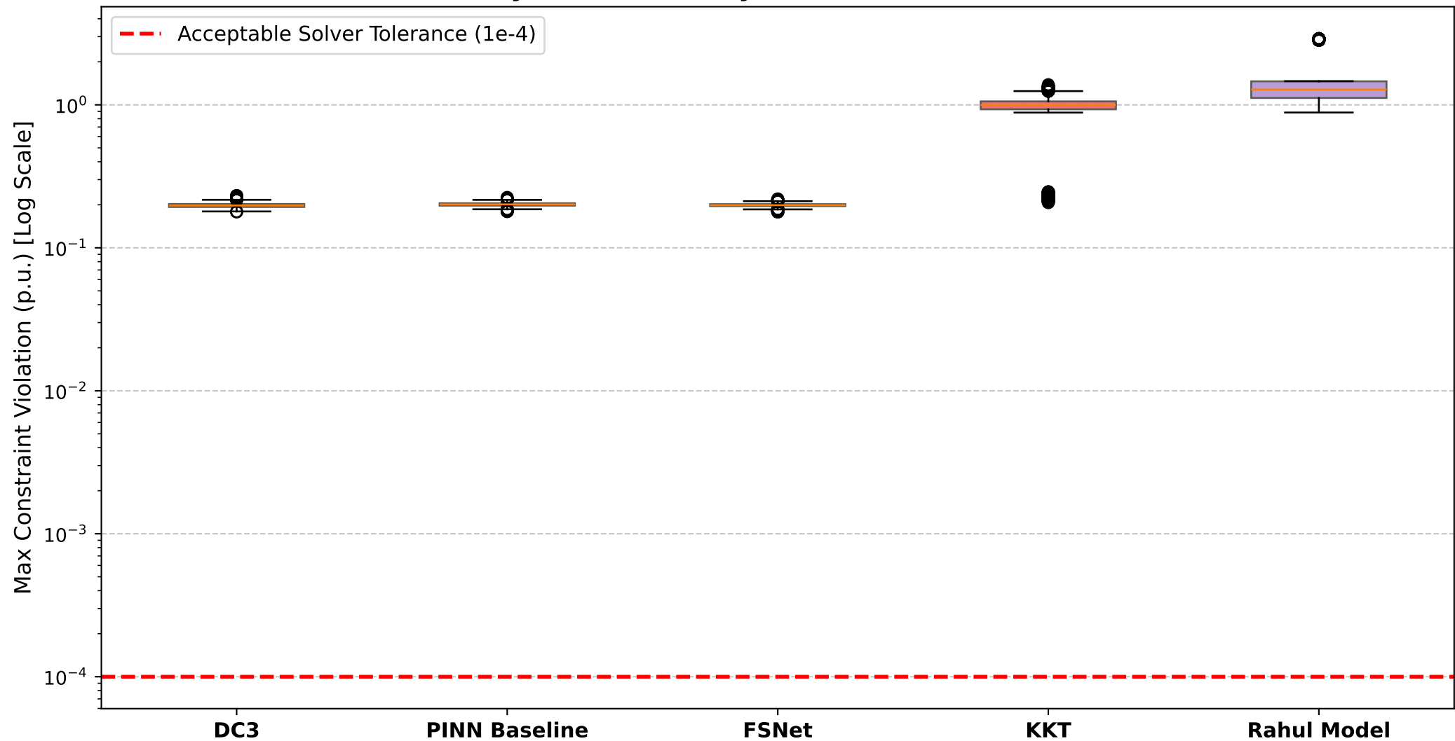
Pooled Physical Feasibility Distribution Across All Seeds
