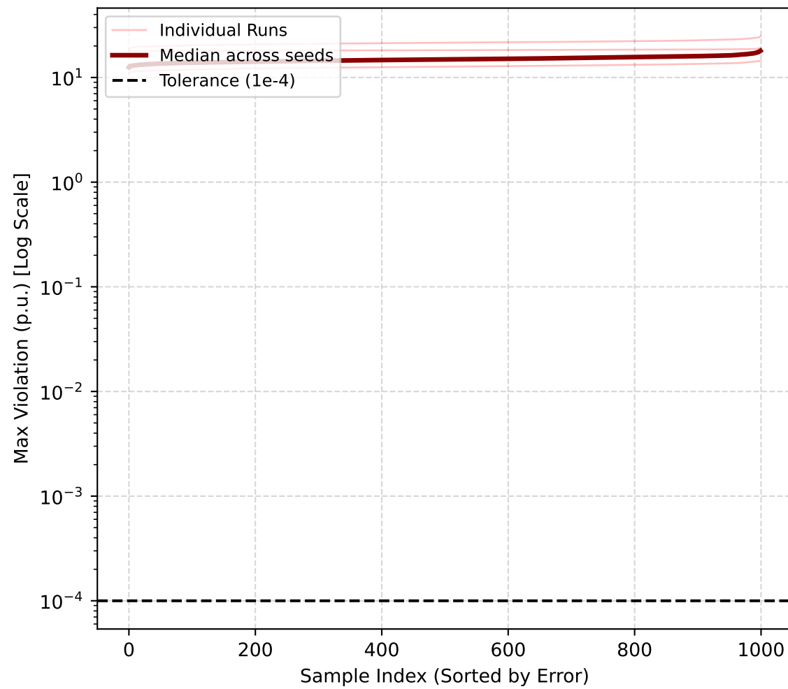
KKT (4 seeds)
