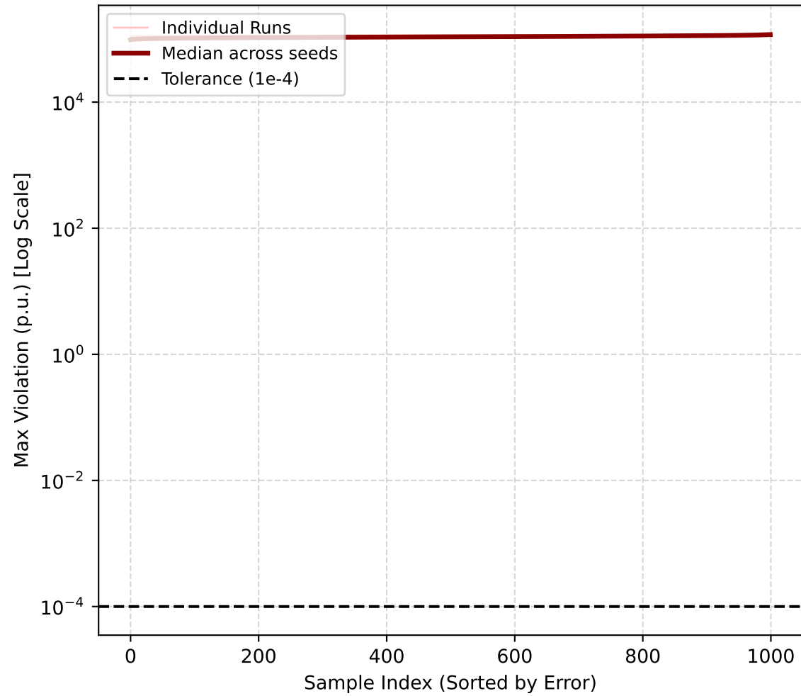
KKT (4 seeds)
