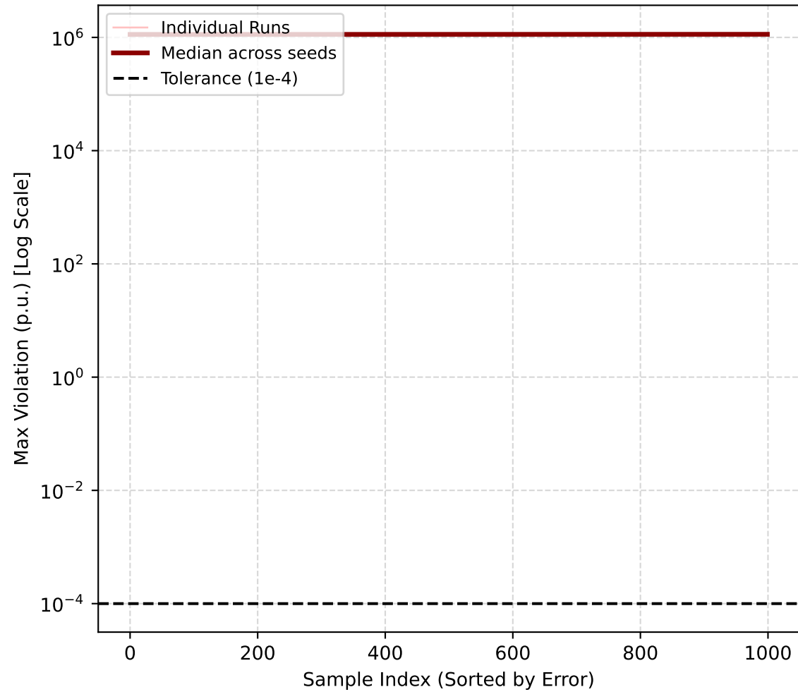
KKT (4 seeds)
