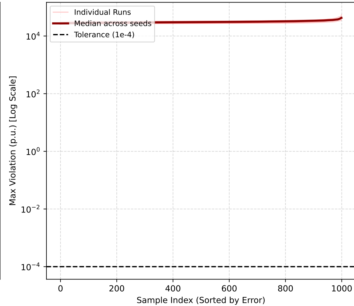
FSNet (5 seeds)
