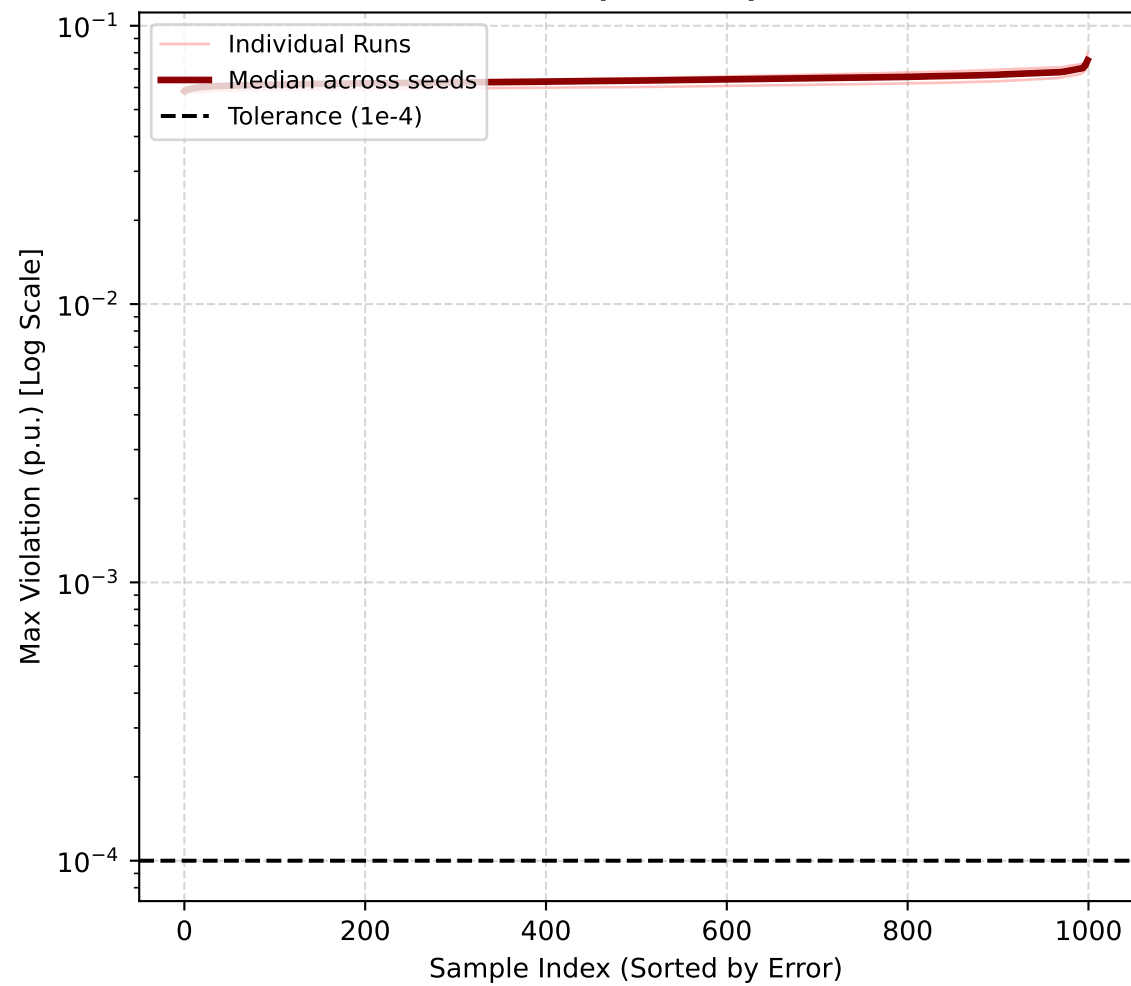
KKT (5 seeds)
