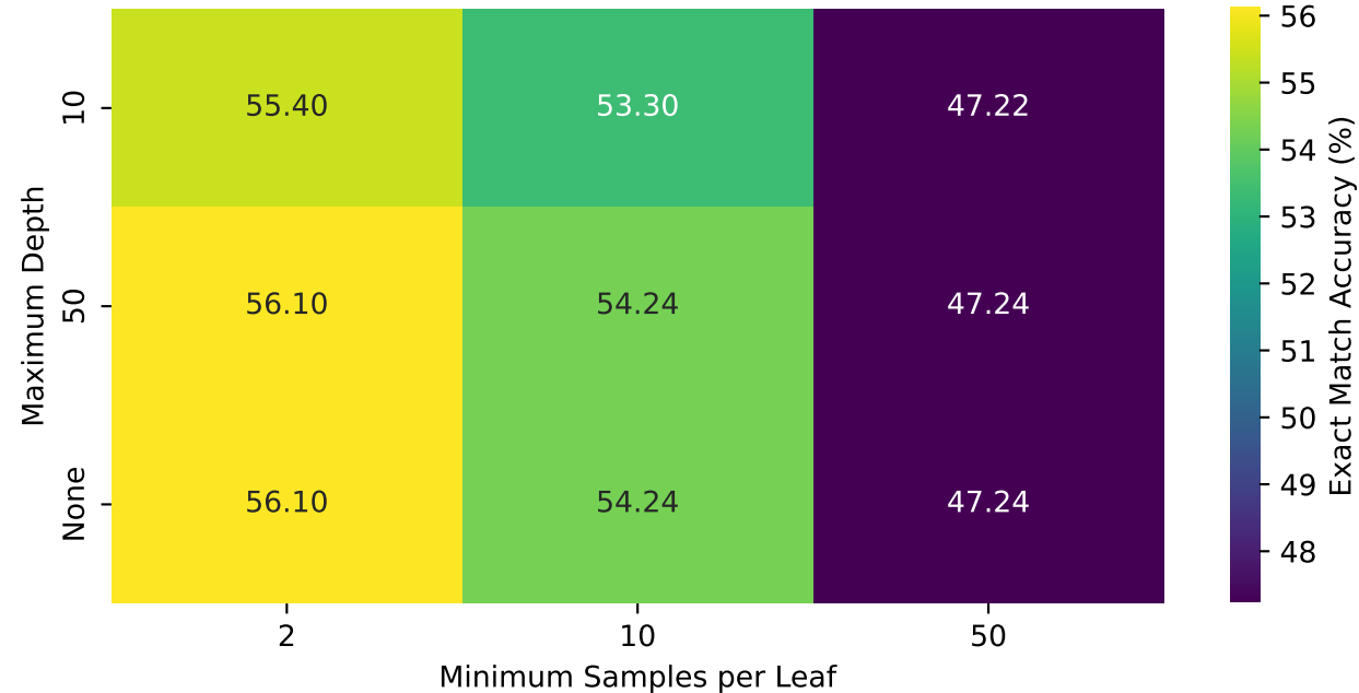
RF Hyperparameter Sensitivity (Averaged over 5 Seeds) pglib_opf_case73_ieee_rts, sigma=0.01
