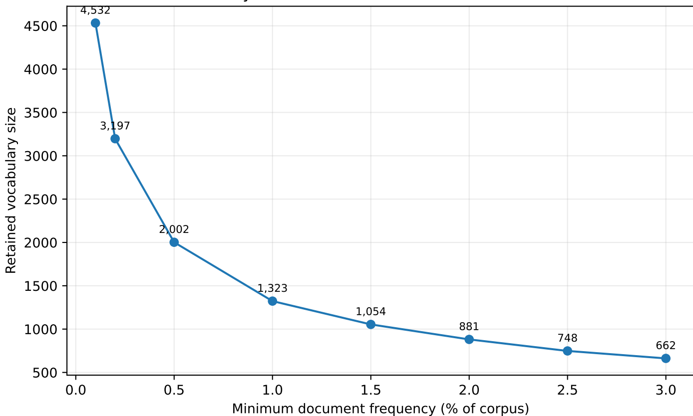
Vocabulary Retention under Alternative DF Thresholds
