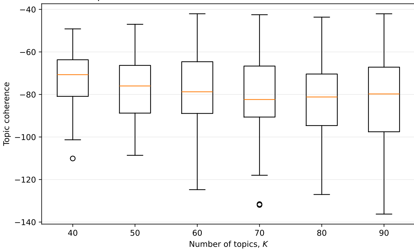
Topic-Coherence Distribution Across Candidate LDA Models
