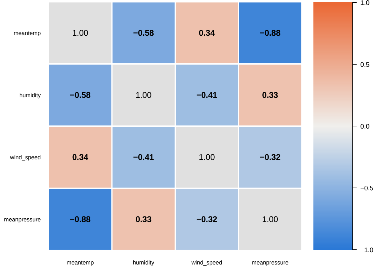
Spearman rho
