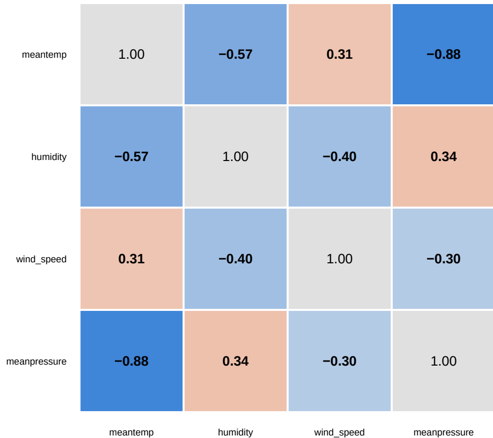
Pearson r
