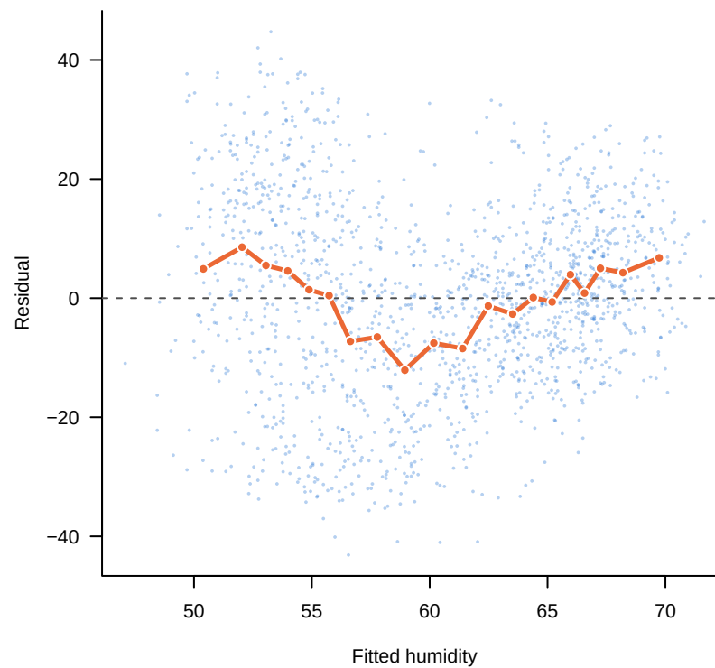
humidity ~ meanpressure (DW = 0.26)
