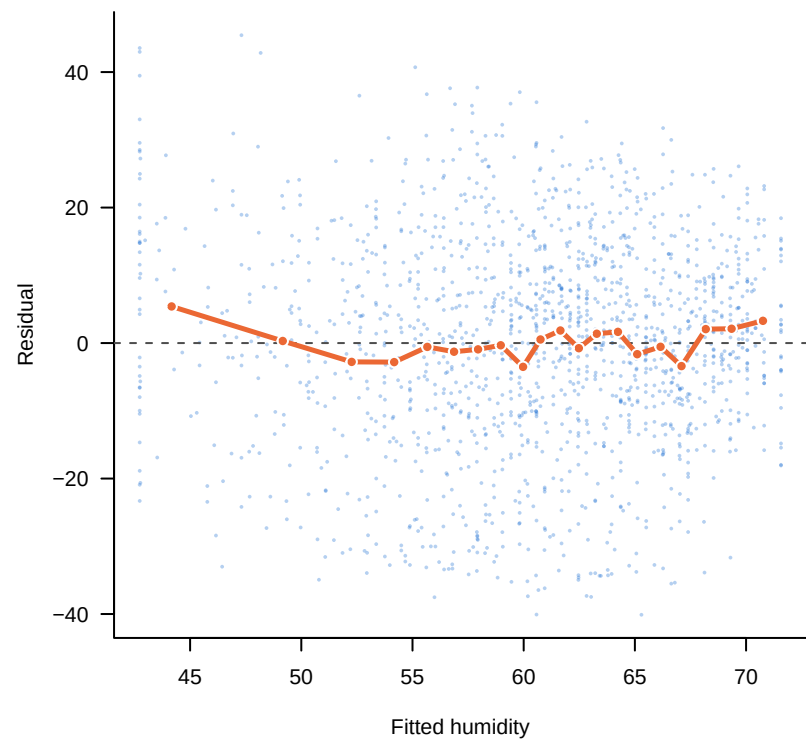
humidity ~ wind_speed (DW = 0.37)
