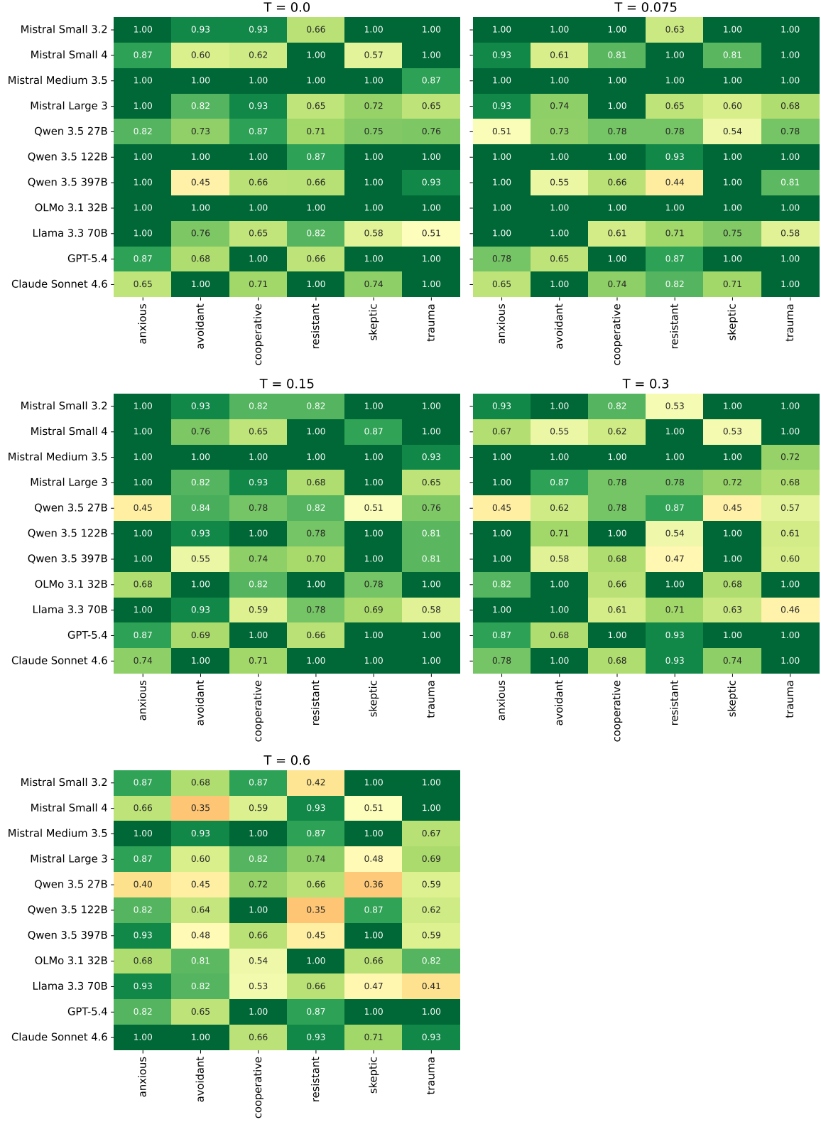
Figure 12: Median Jaccard per model × vignette, one heatmap per temperature. Individual model–vignette combinations can deviate noticeably from the aggregate even though the overall vignette effect is not significant (Section 5.4).
